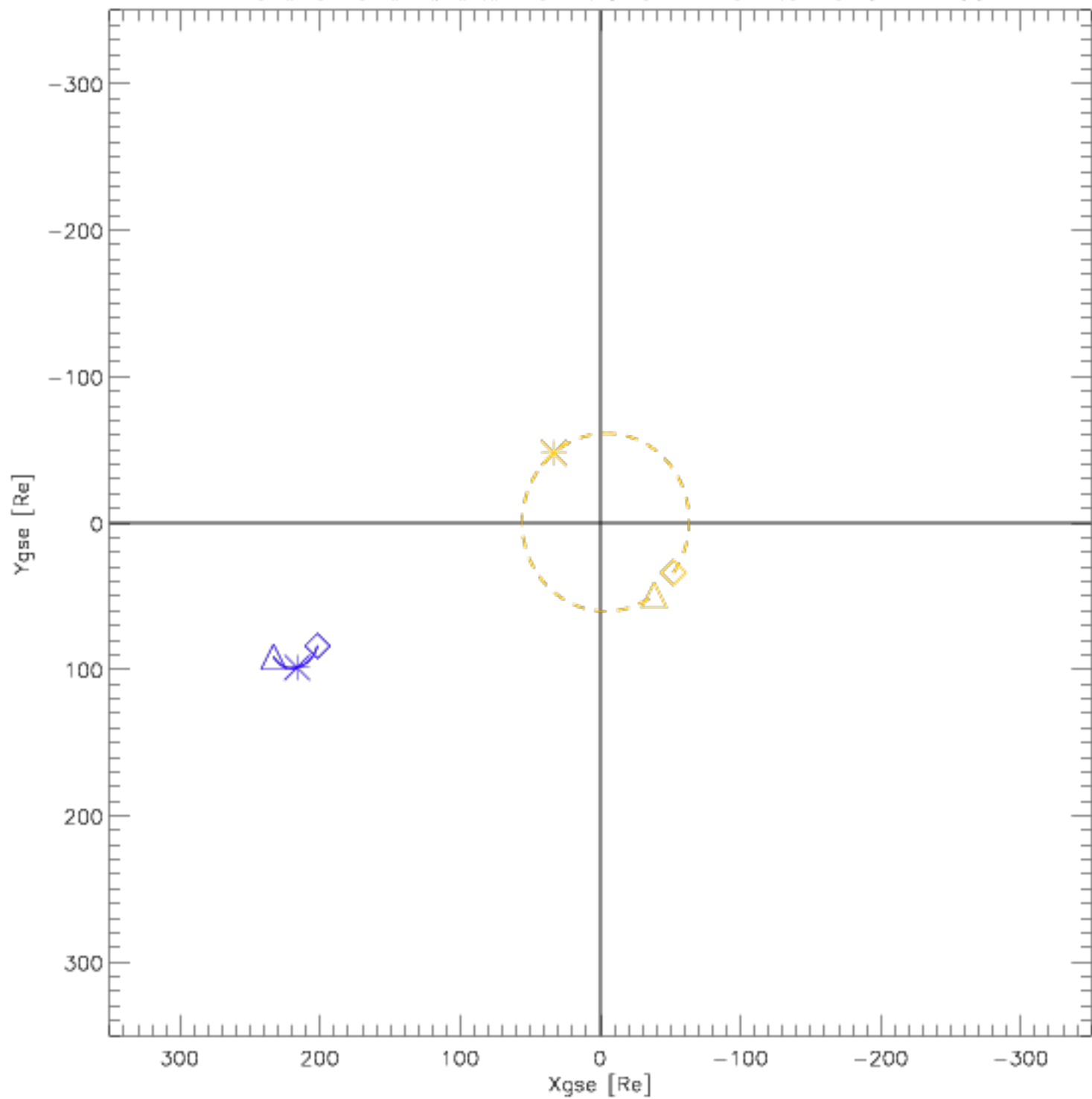
Wind and Lunar Orbits from 2016-11-01 to 2016-11-30
