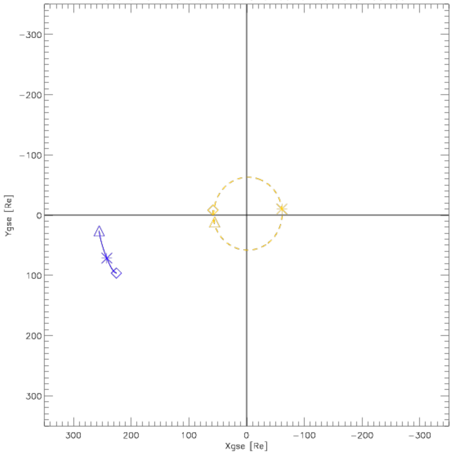
Wind and Lunar Orbits from 2016-06-01 to 2016-06-30
