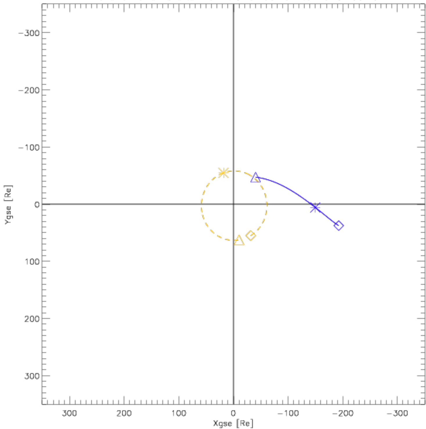
Wind and Lunar Orbits from 2016-05-01 to 2016-05-31
