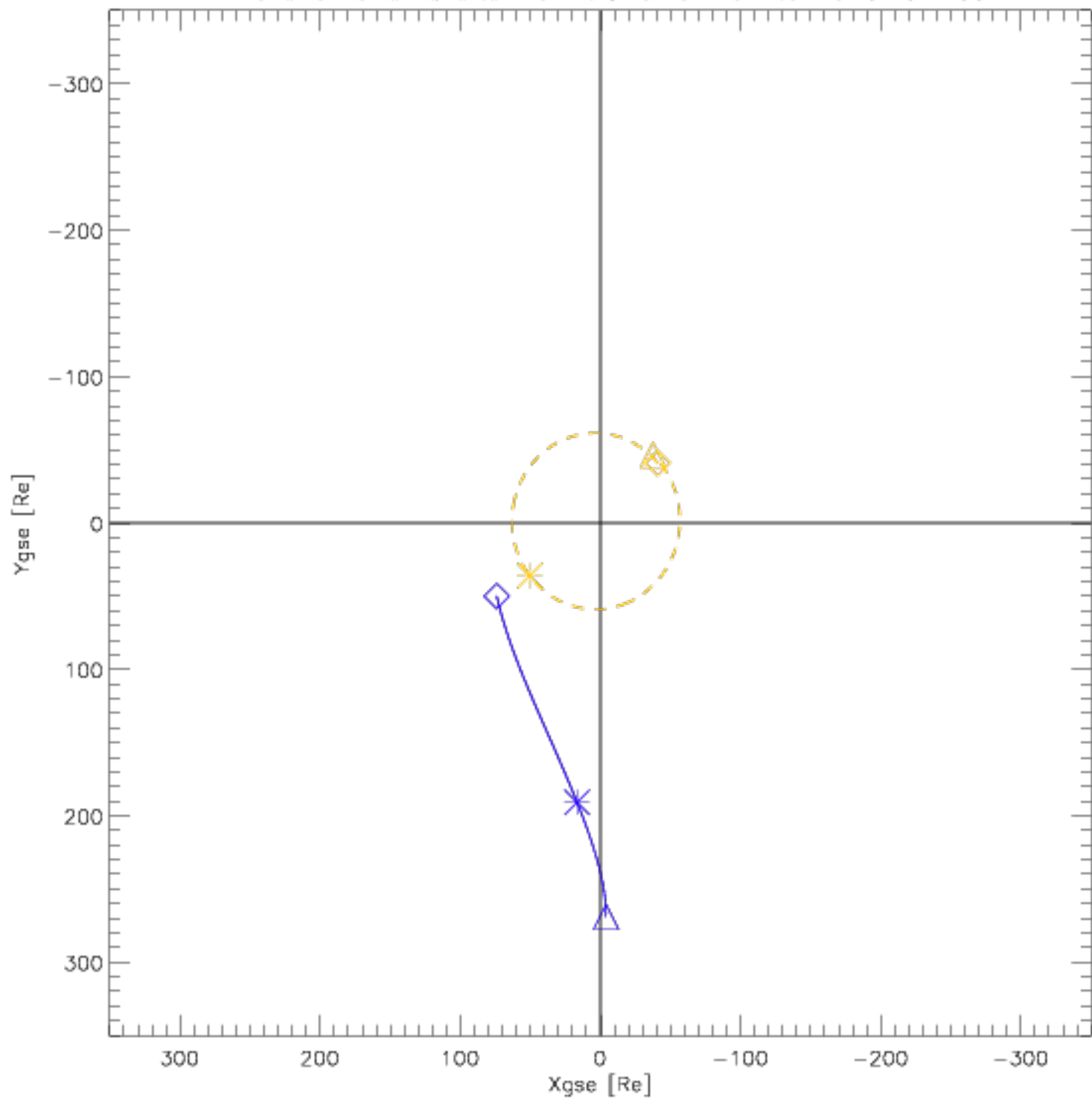
Wind and Lunar Orbits from 2016-04-01 to 2016-04-30
