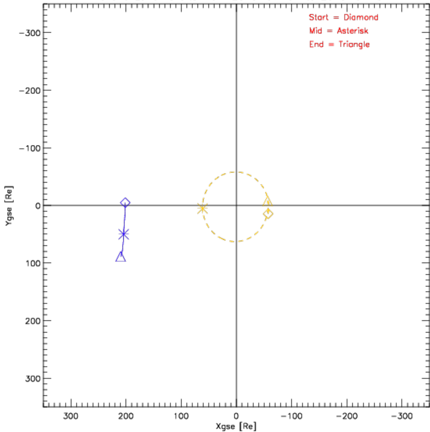
Wind and Lunar Orbits from 2015-07-01 to 2015-07-31
