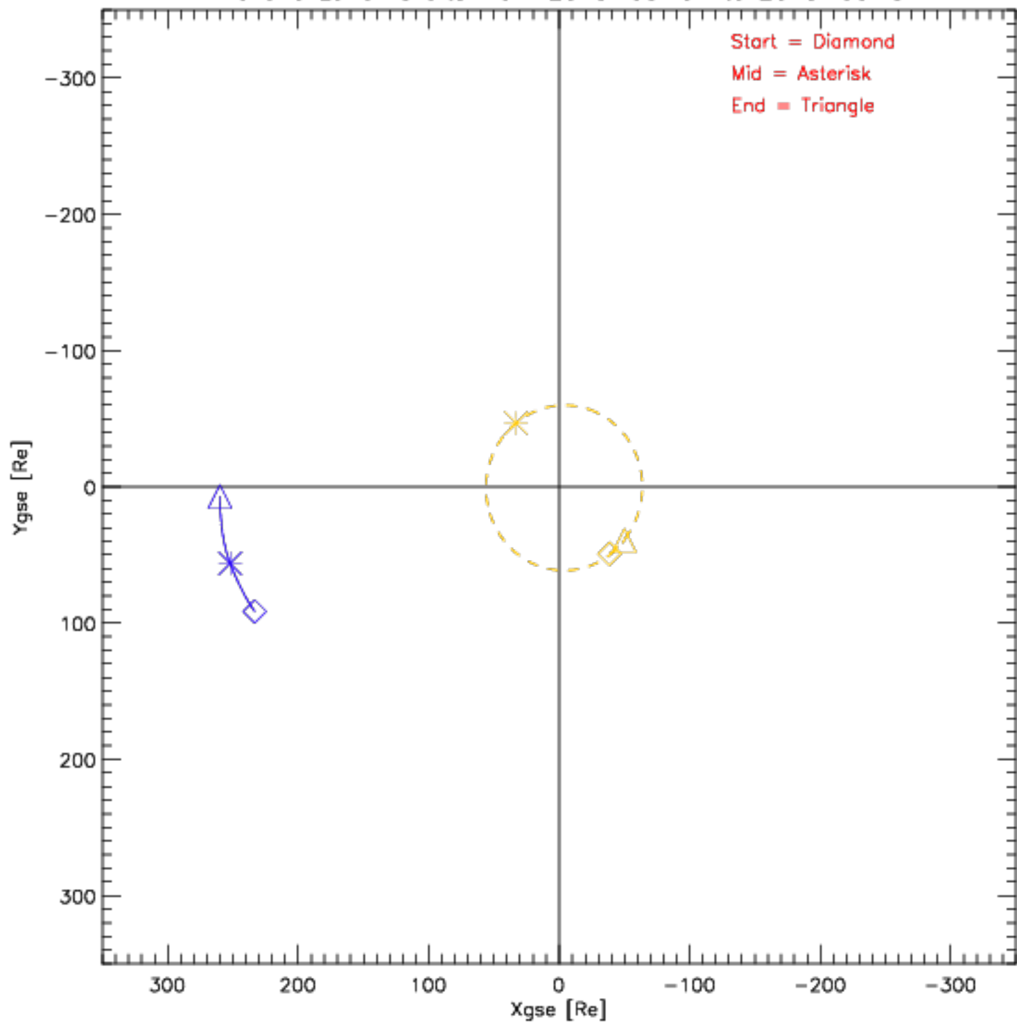
Wind and Lunar Orbits from 2015-03-01 to 2015-03-31
