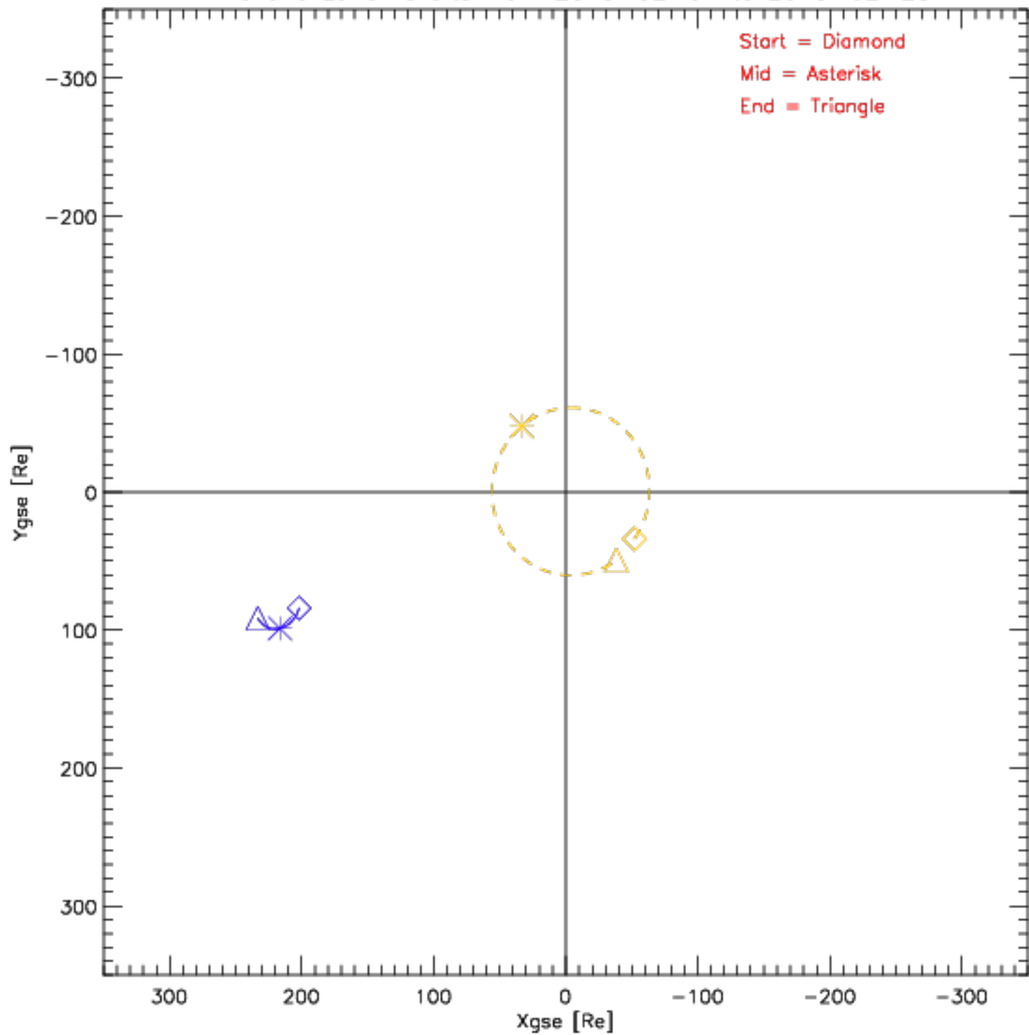
Wind and Lunar Orbits from 2015-02-01 to 2015-02-28
