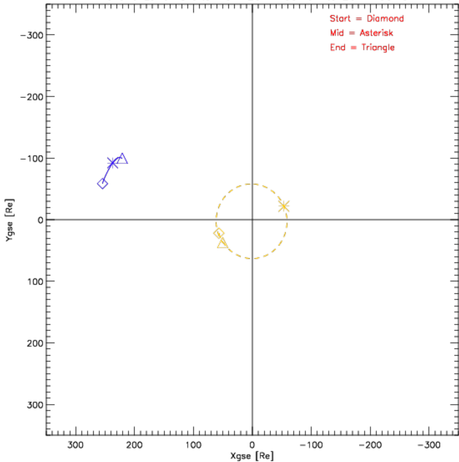
Wind and Lunar Orbits from 2014-05-01 to 2014-05-31
