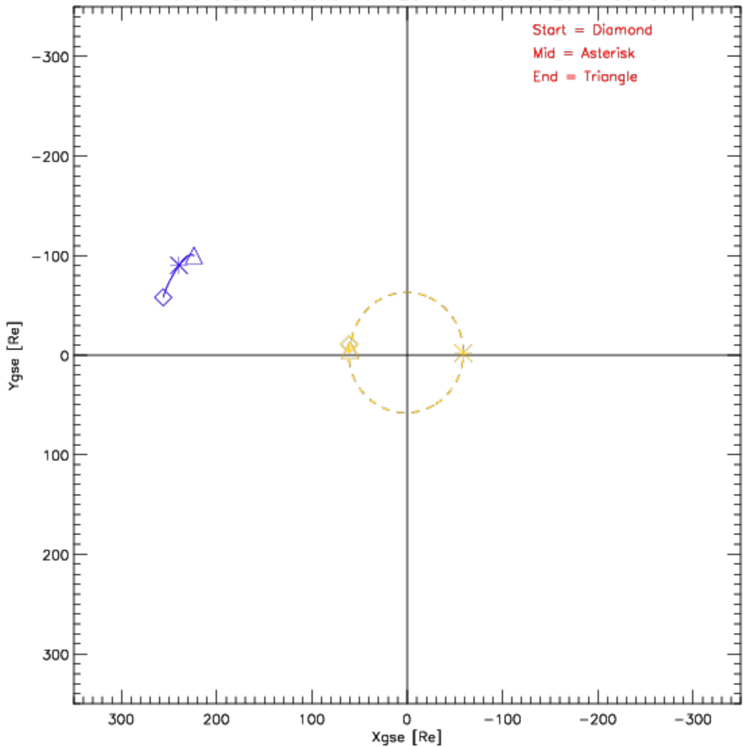
Wind and Lunar Orbits from 2011-06-01 to 2011-06-30
