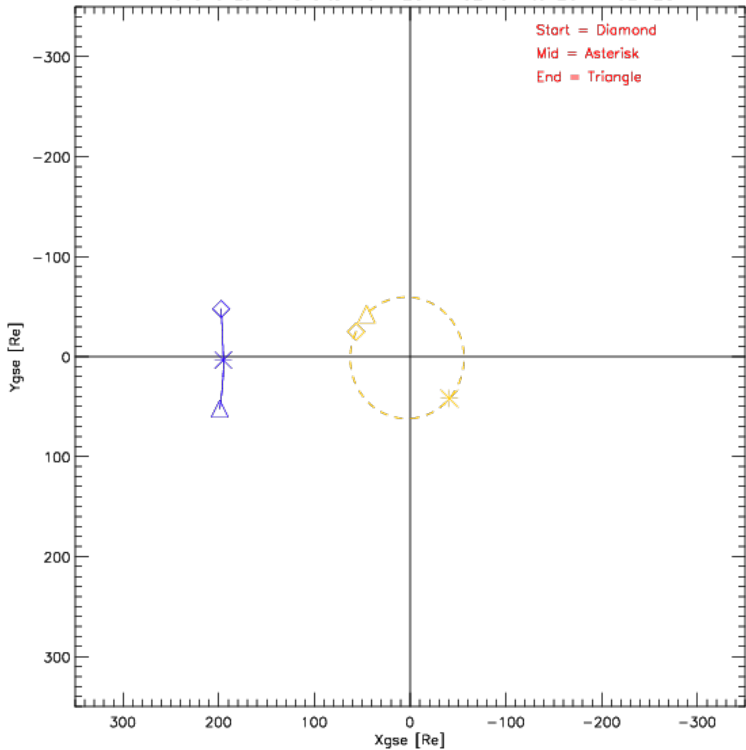
Wind and Lunar Orbits from 2011-02-01 to 2011-02-28
