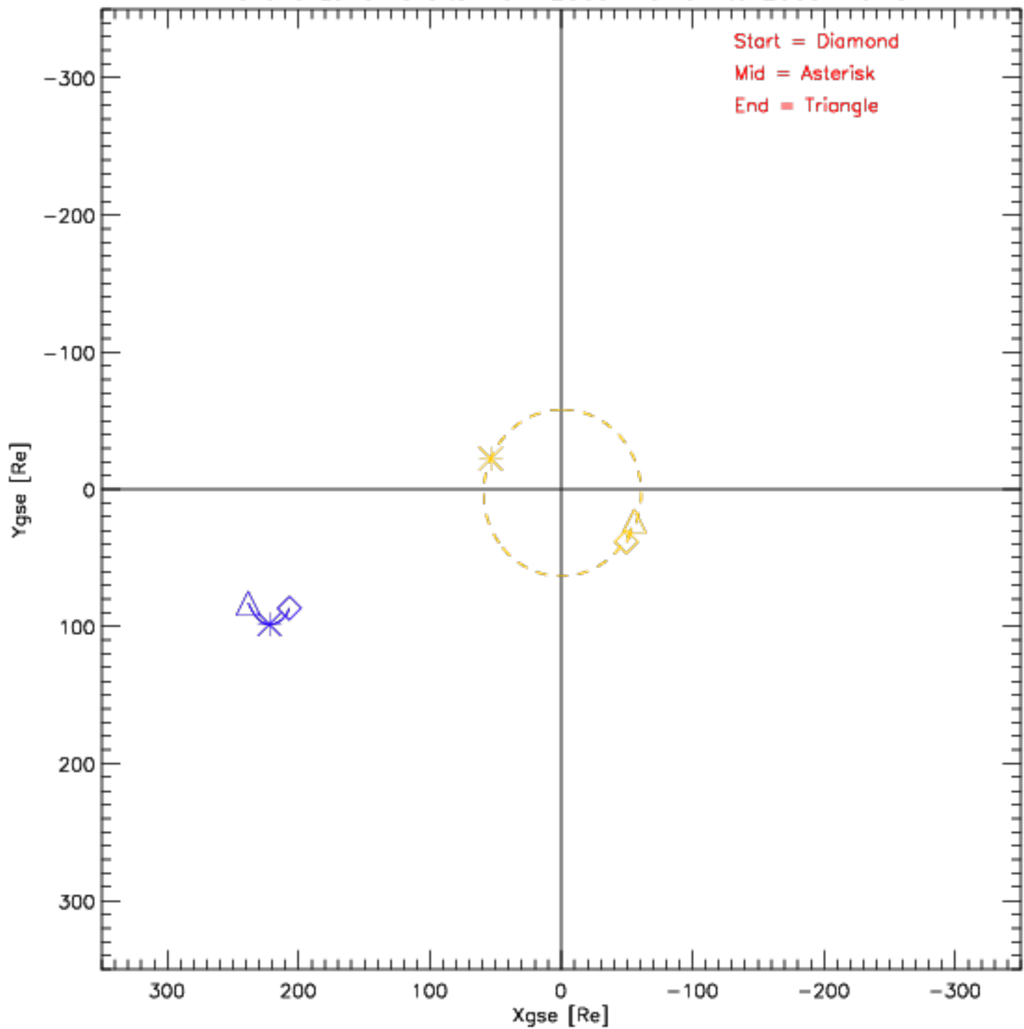
Wind and Lunar Orbits from 2009-10-01 to 2009-10-31
