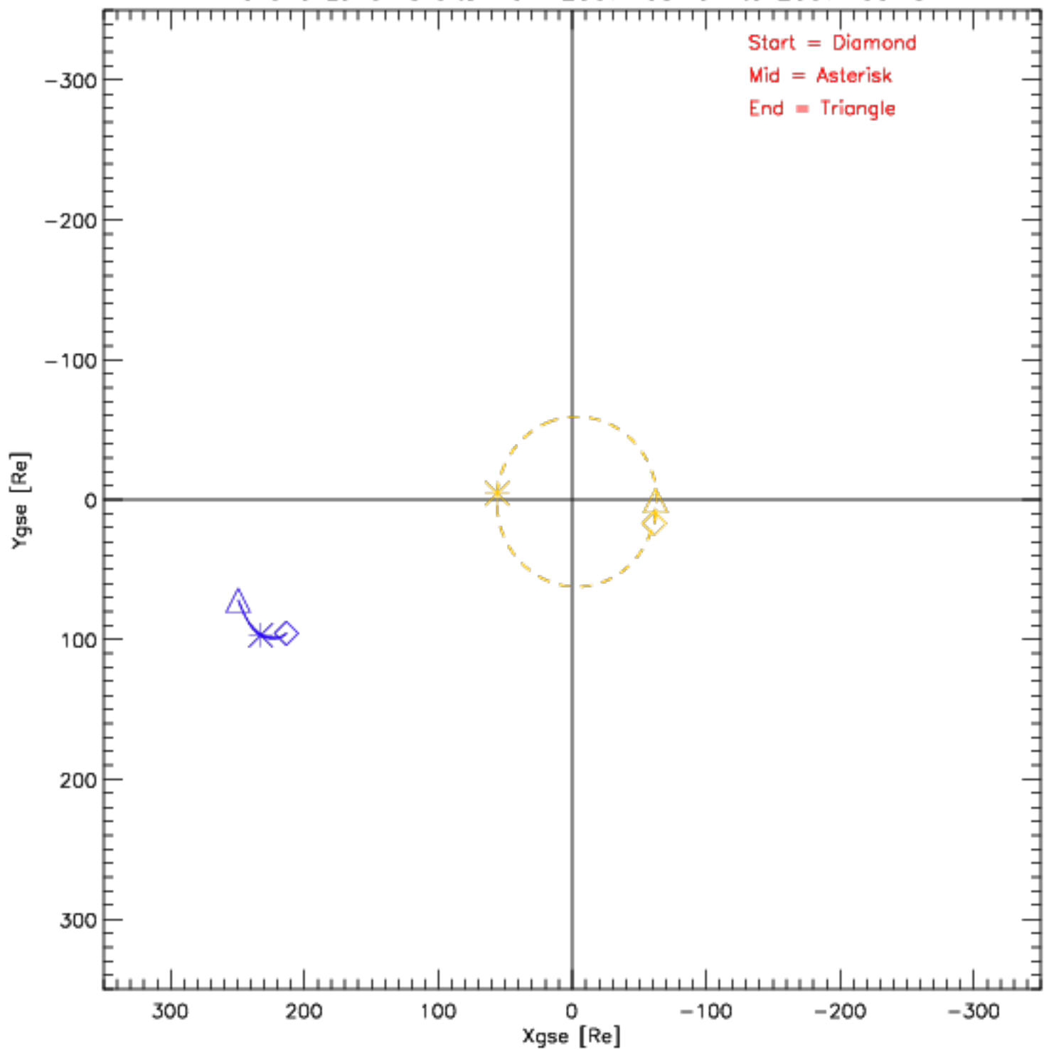
Wind and Lunar Orbits from 2007-05-01 to 2007-05-31
