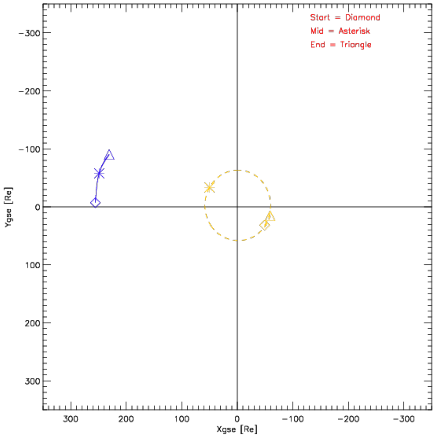
Wind and Lunar Orbits from 2007-01-01 to 2007-01-31
