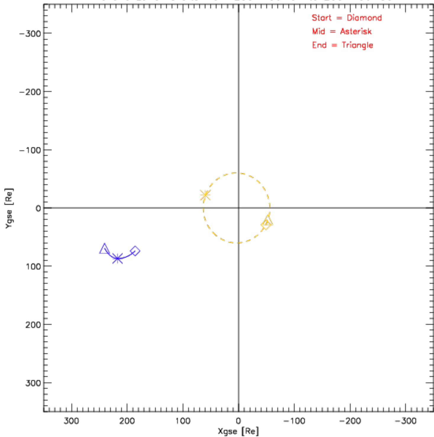
Wind and Lunar Orbits from 2004-06-01 to 2004-06-30
