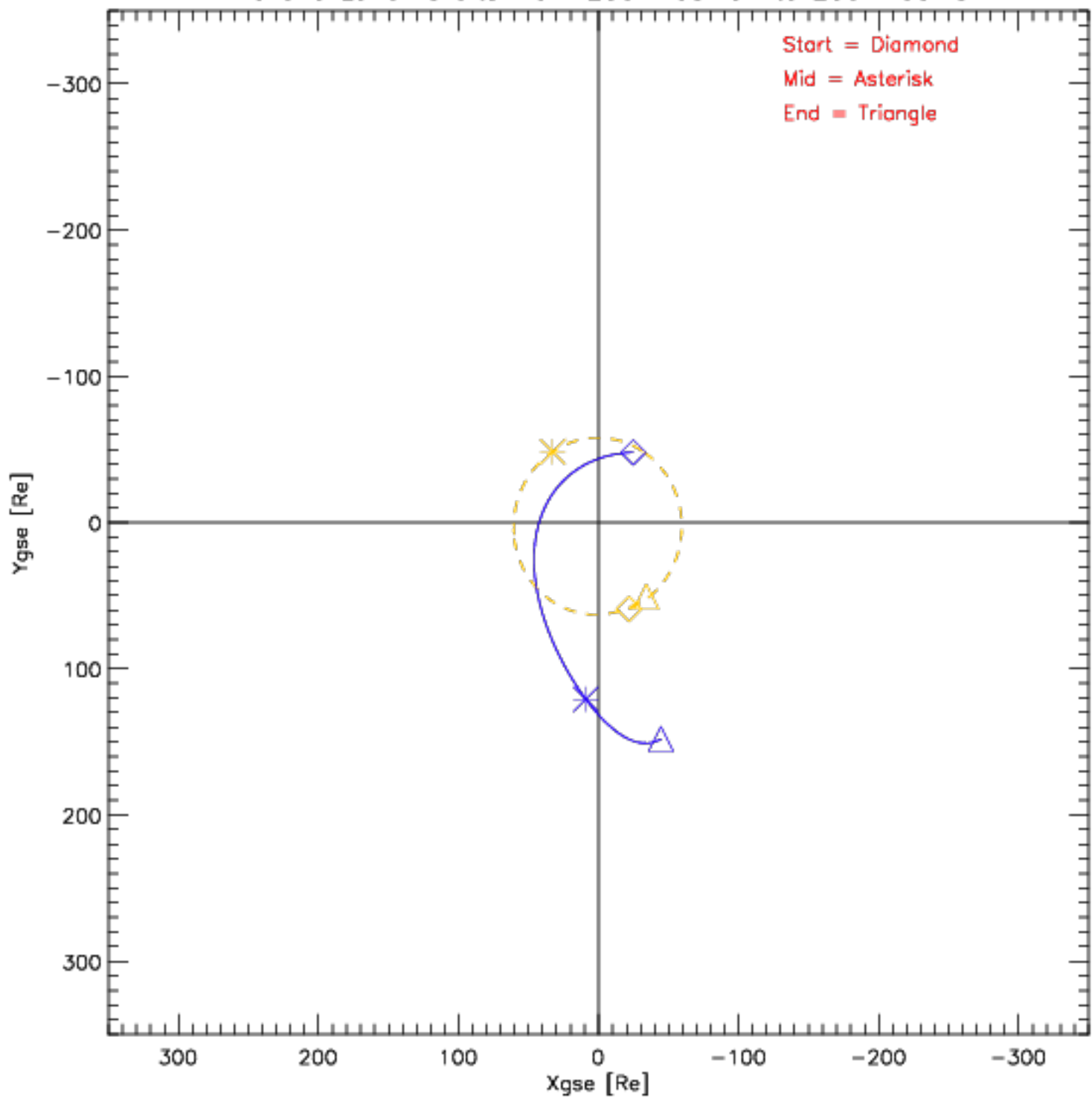
Wind and Lunar Orbits from 2004-03-01 to 2004-03-31
