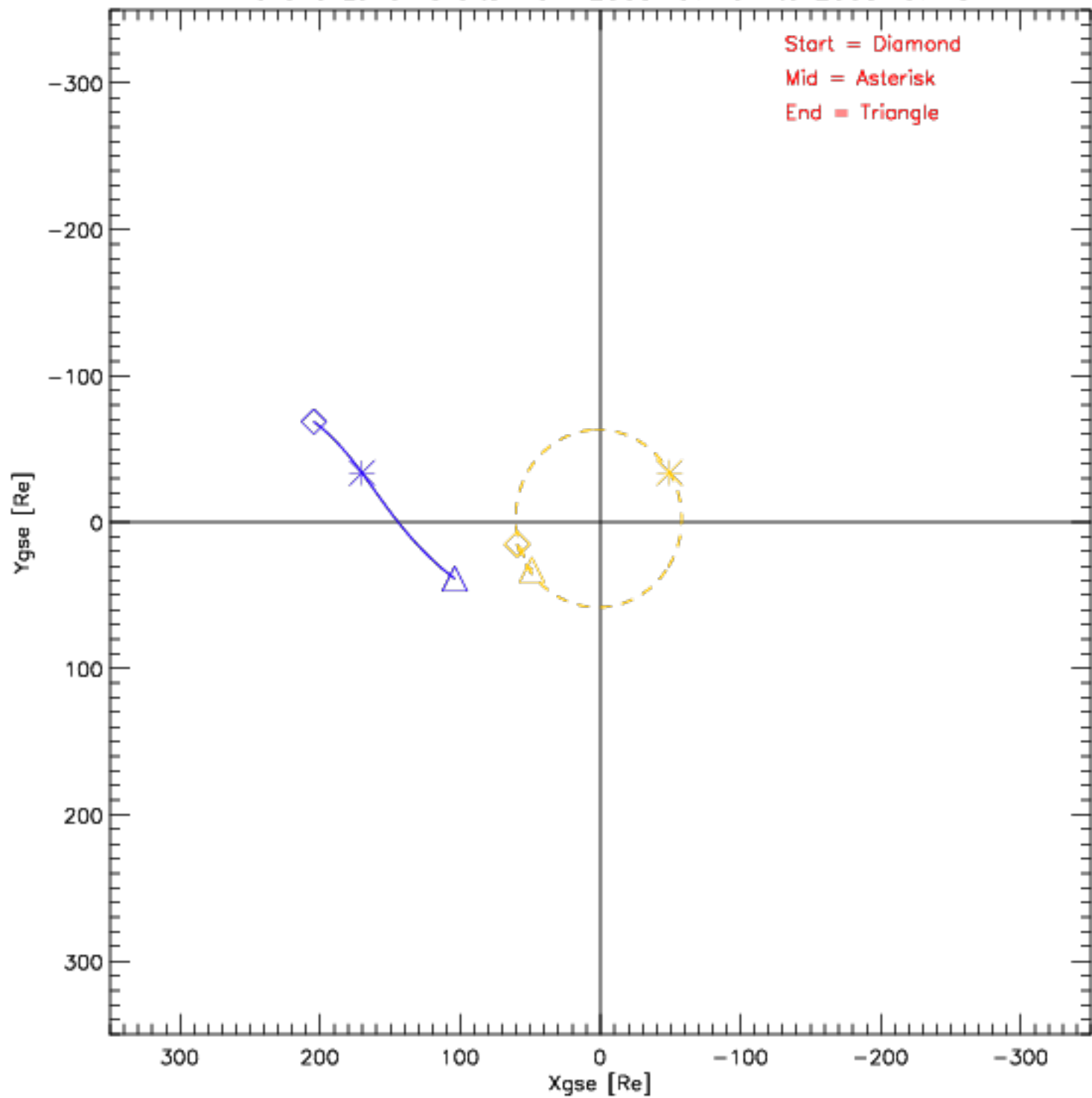
Wind and Lunar Orbits from 2003-07-01 to 2003-07-31
