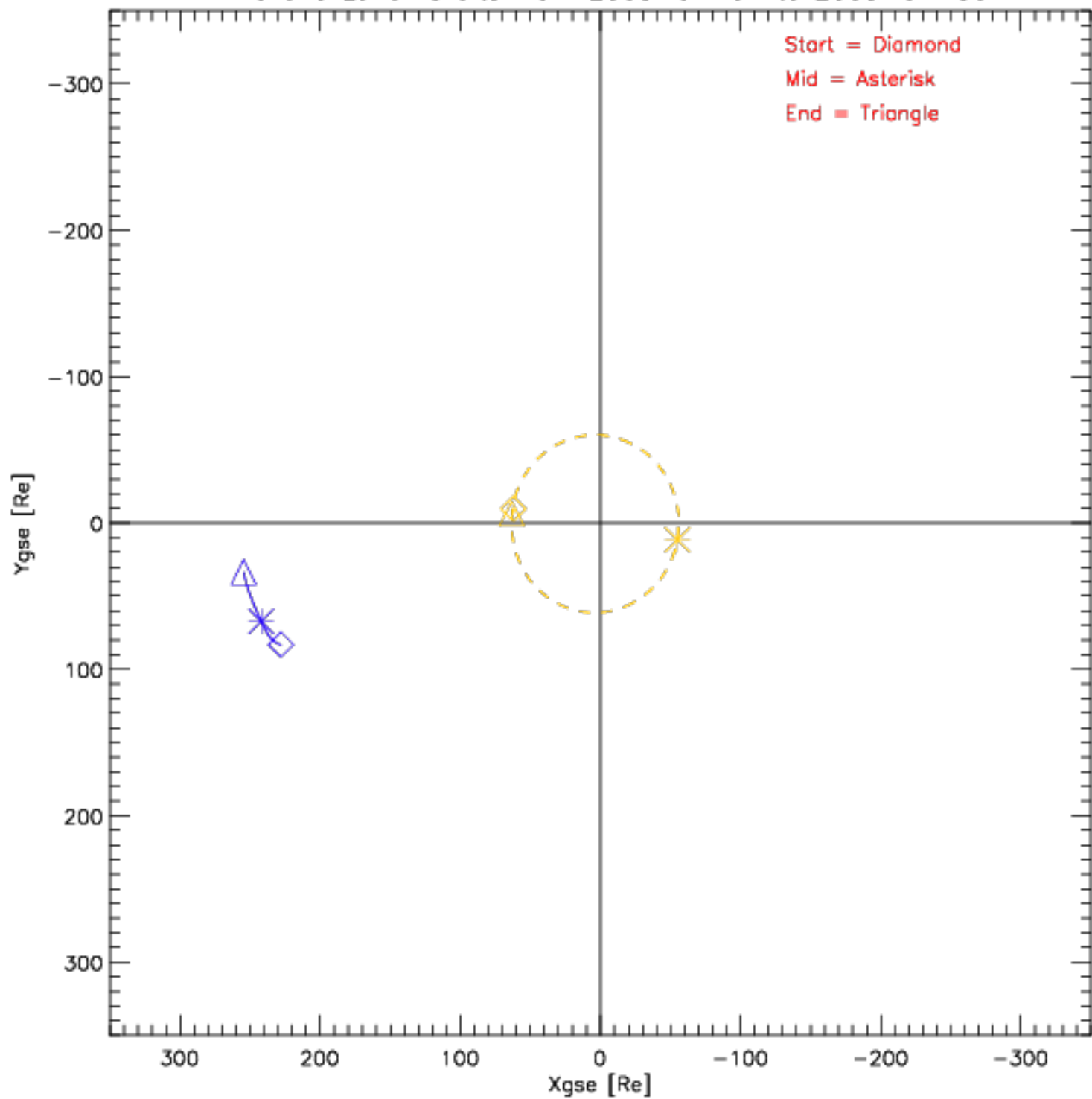
Wind and Lunar Orbits from 2003-04-01 to 2003-04-30
