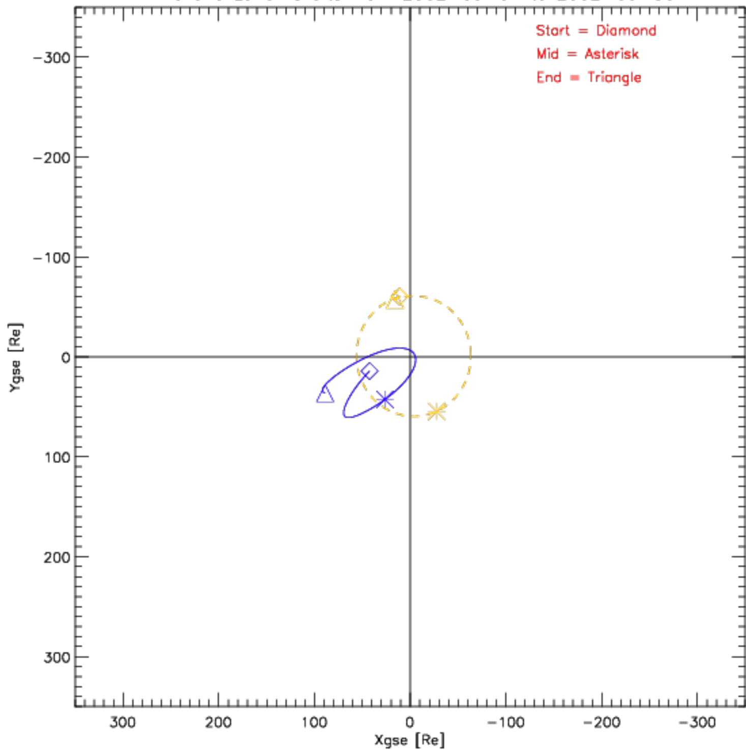
Wind and Lunar Orbits from 2002-09-01 to 2002-09-30
