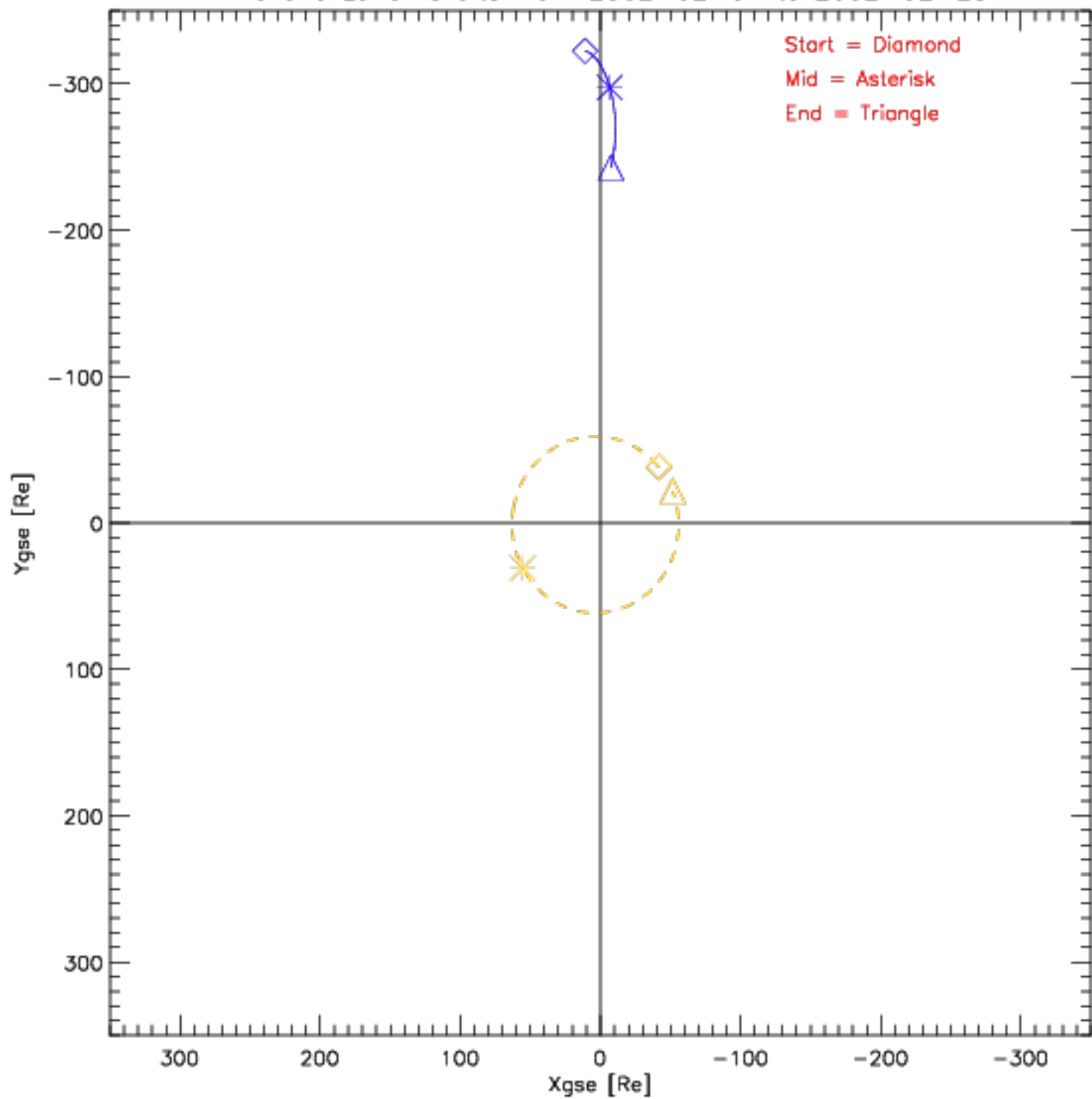
Wind and Lunar Orbits from 2002-02-01 to 2002-02-28
