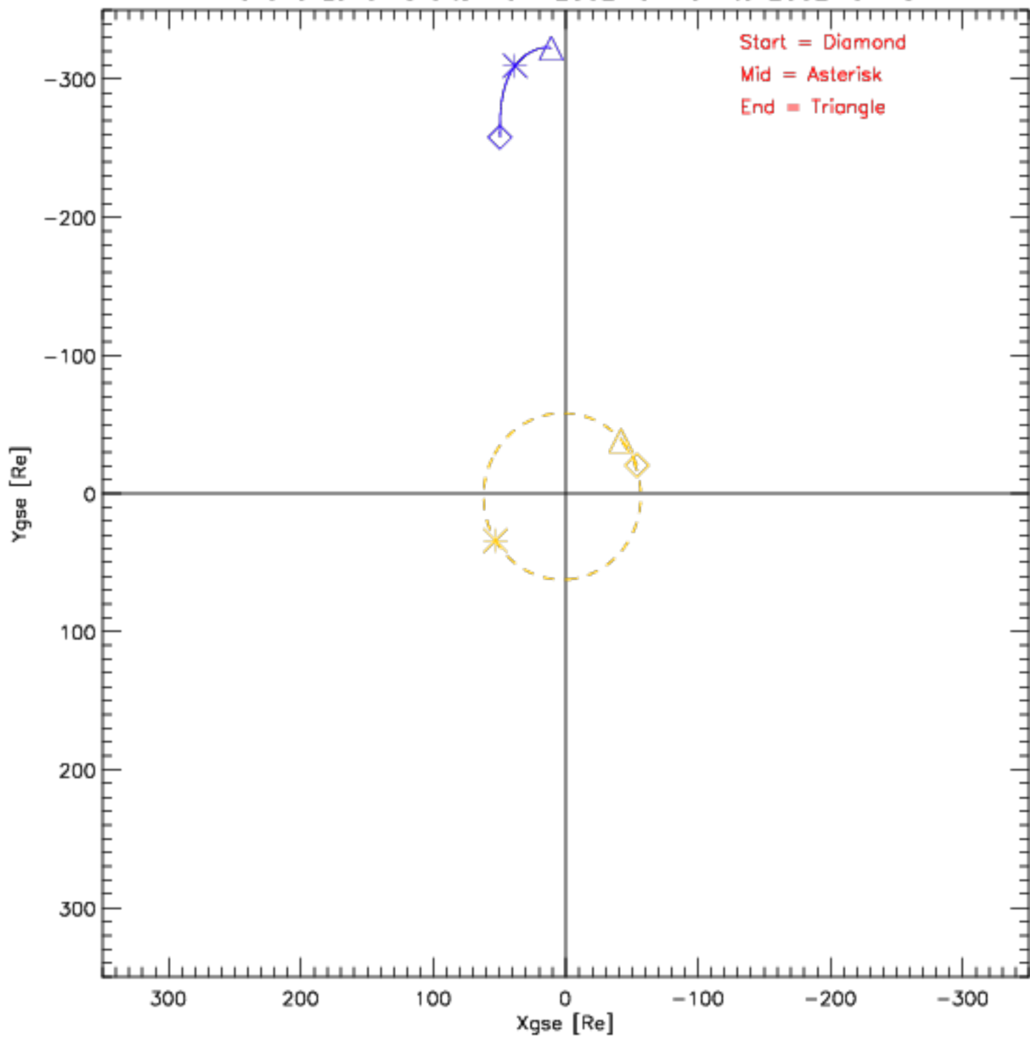
Wind and Lunar Orbits from 2002-01-01 to 2002-01-31
