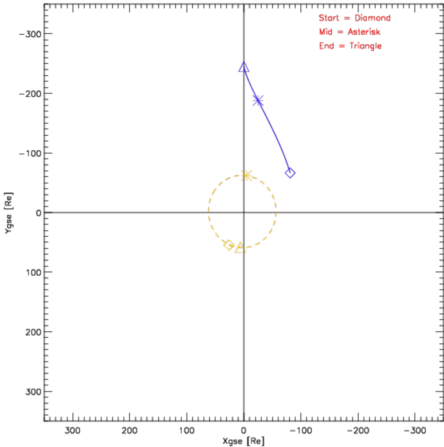
Wind and Lunar Orbits from 2001-03-01 to 2001-03-31
