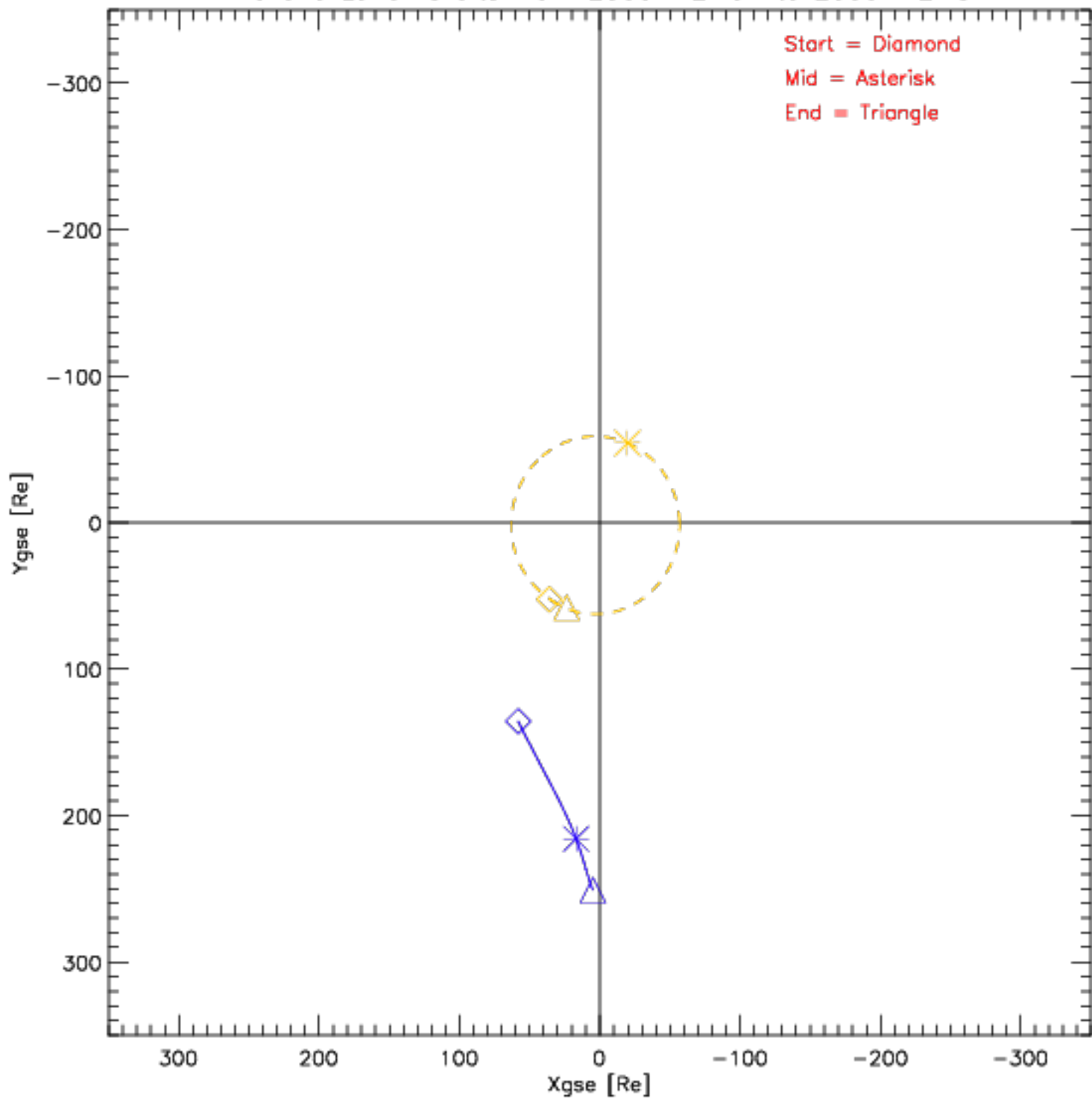
Wind and Lunar Orbits from 2000-12-01 to 2000-12-31
