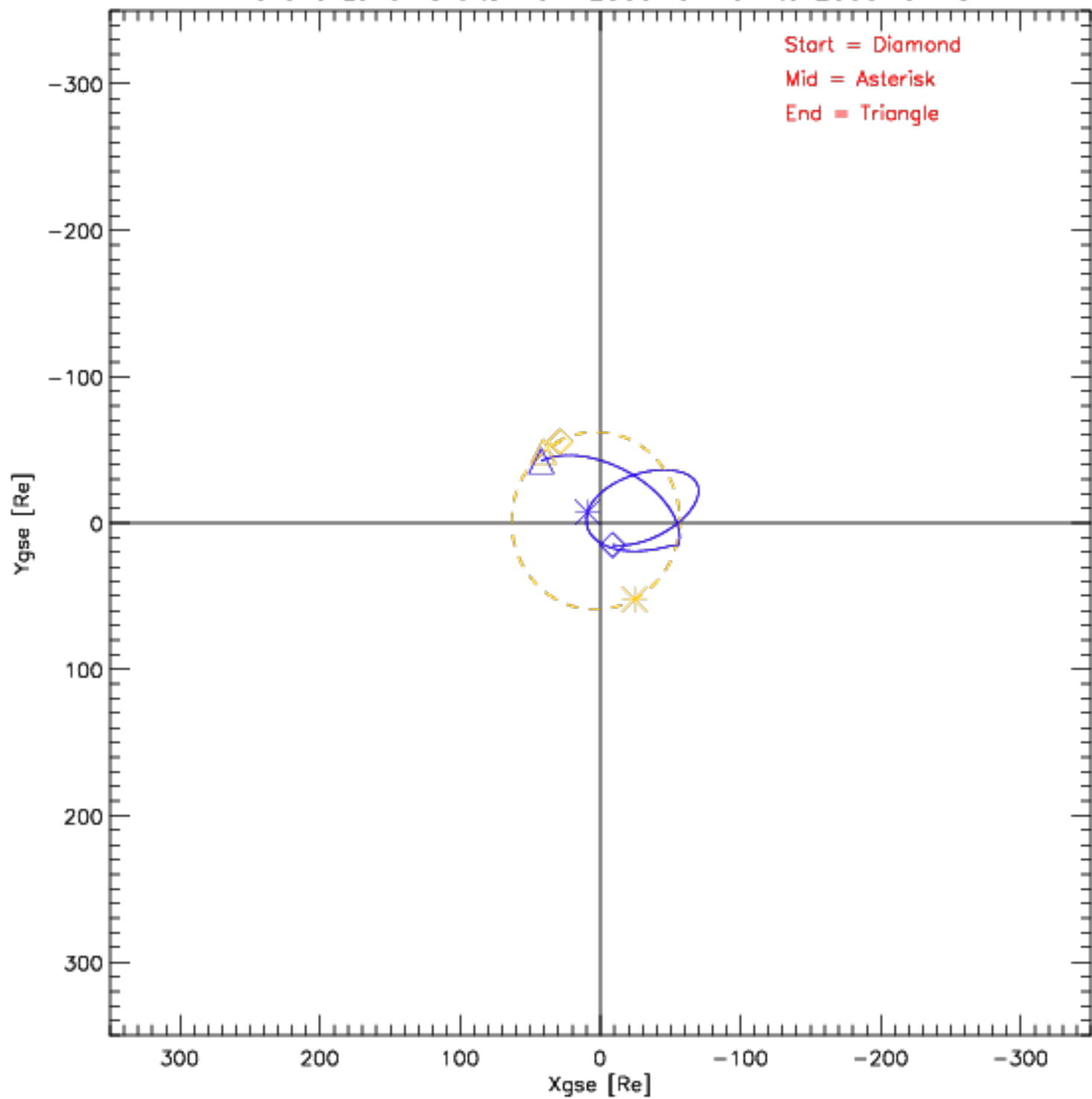
Wind and Lunar Orbits from 2000-01-01 to 2000-01-31
