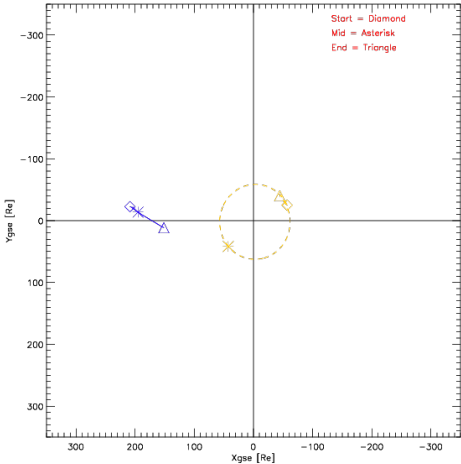
Wind and Lunar Orbits from 1999-07-01 to 1999-07-31
