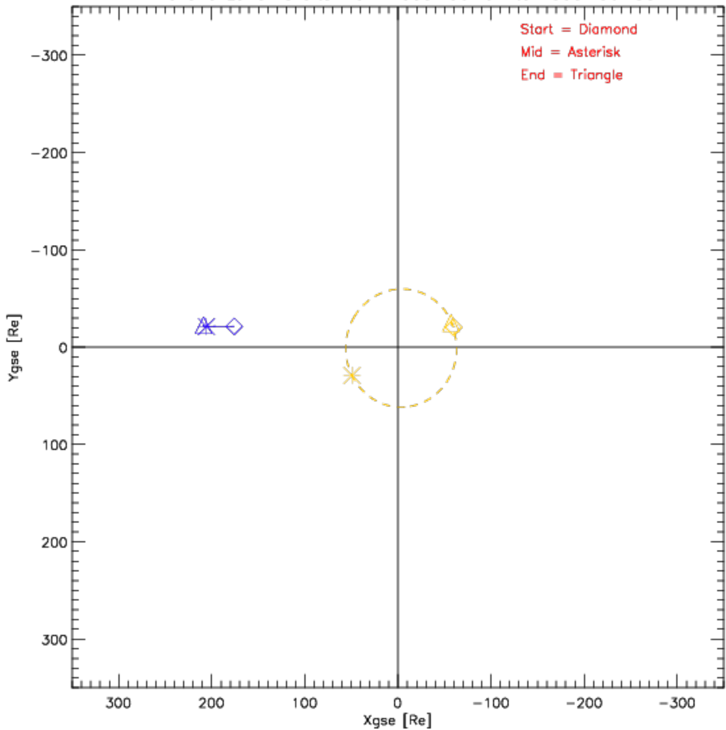
Wind and Lunar Orbits from 1999-06-01 to 1999-06-30
