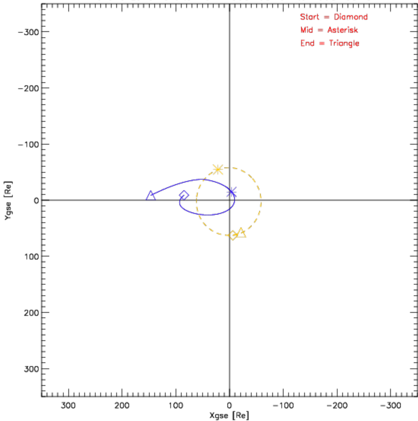
Wind and Lunar Orbits from 1998-08-01 to 1998-08-31
