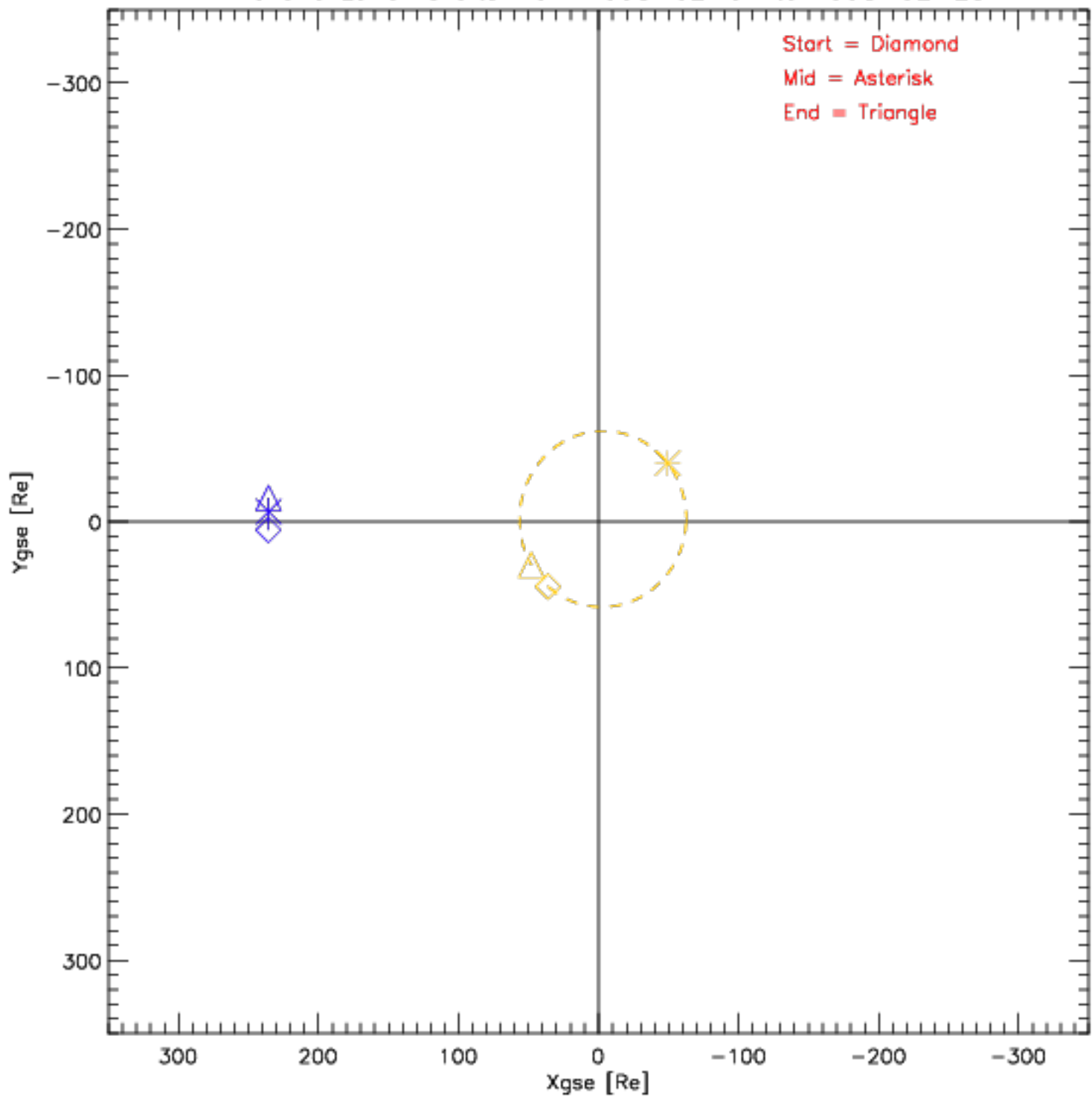
Wind and Lunar Orbits from 1998-02-01 to 1998-02-28
