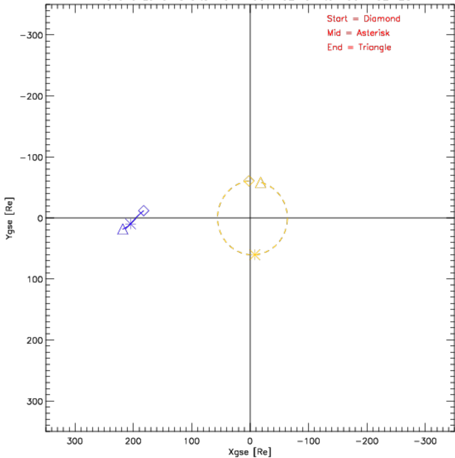
Wind and Lunar Orbits from 1997-02-01 to 1997-02-28
