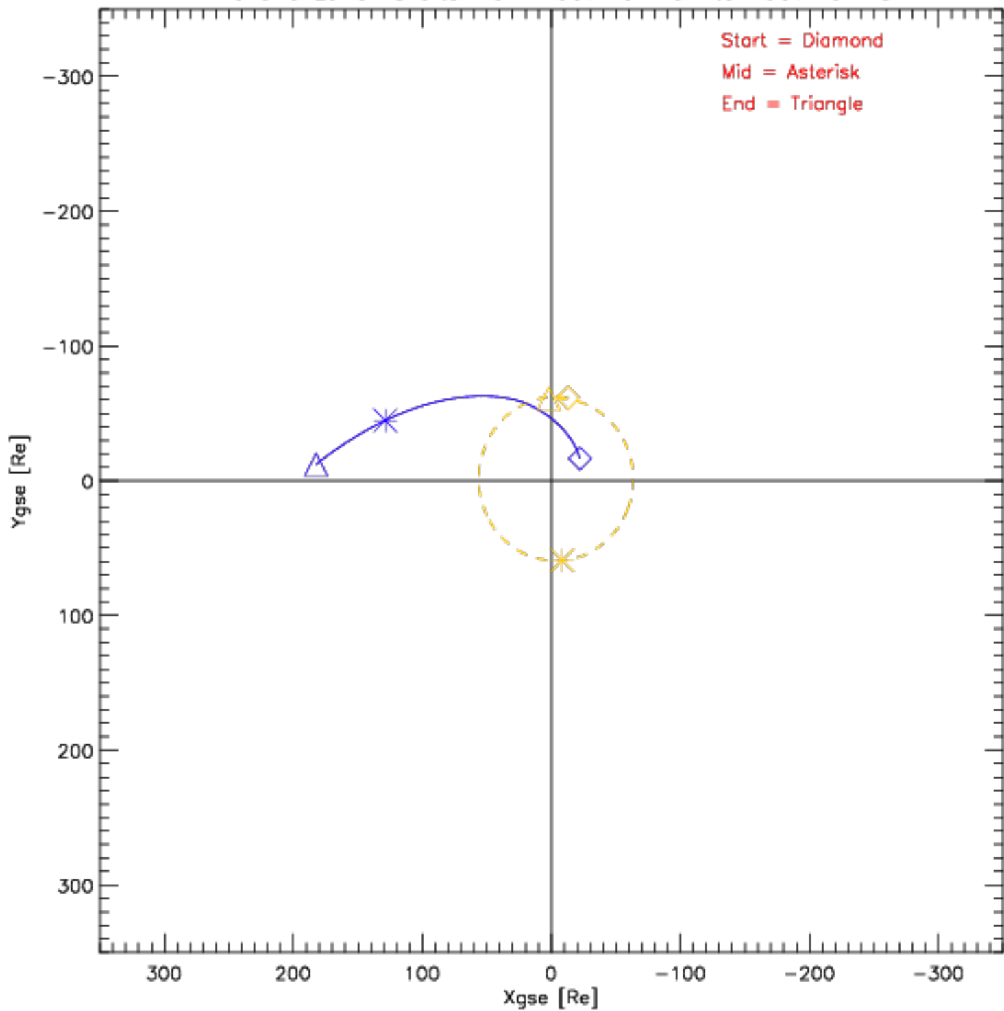
Wind and Lunar Orbits from 1997-01-01 to 1997-01-31
