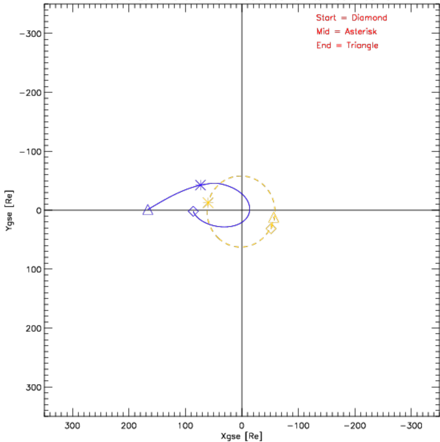
Wind and Lunar Orbits from 1996-05-01 to 1996-05-31
