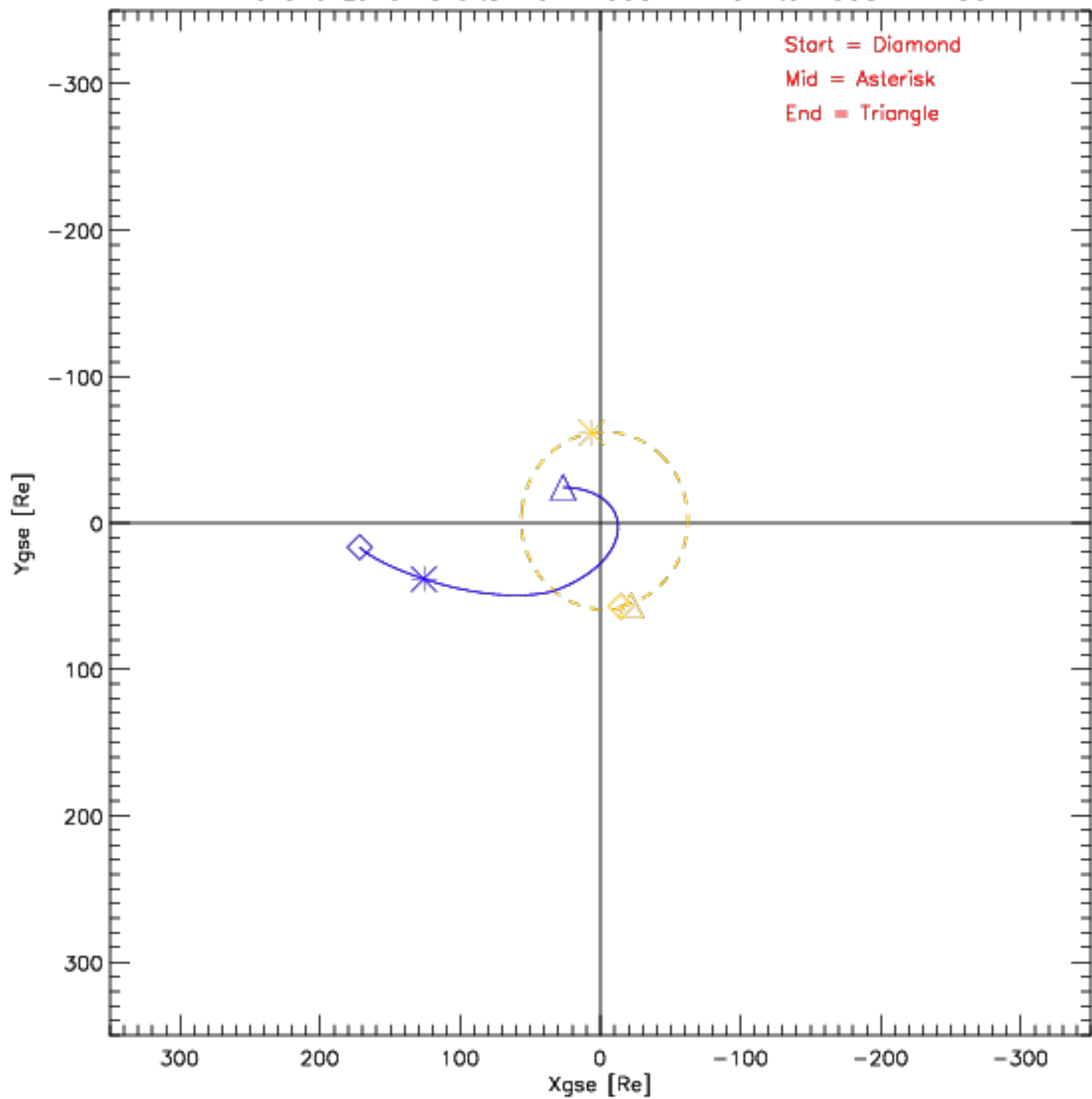
Wind and Lunar Orbits from 1995-11-01 to 1995-11-30
