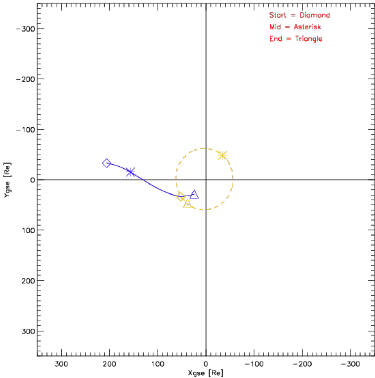
Wind and Lunar Orbits from 1995-07-01 to 1995-07-31
