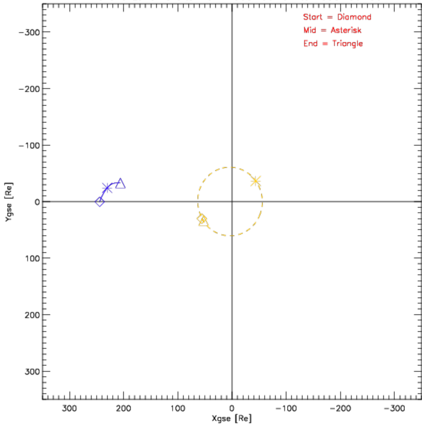
Wind and Lunar Orbits from 1995-06-01 to 1995-06-30
