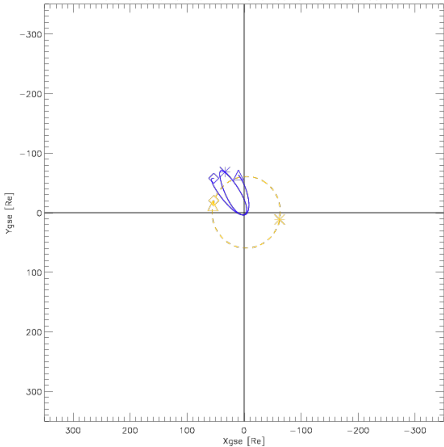
Wind and Lunar Orbits from 2016-03-01 to 2016-03-31
