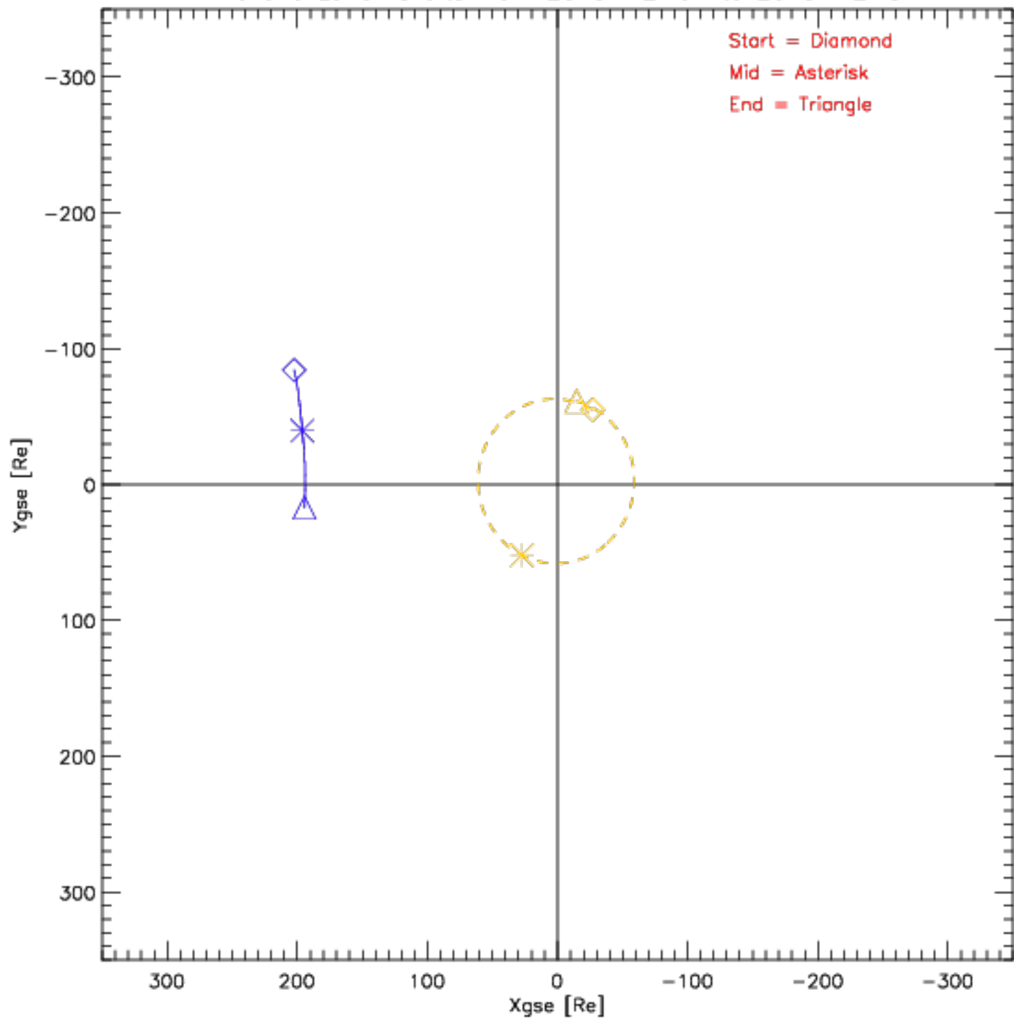
Wind and Lunar Orbits from 2015-12-01 to 2015-12-31
