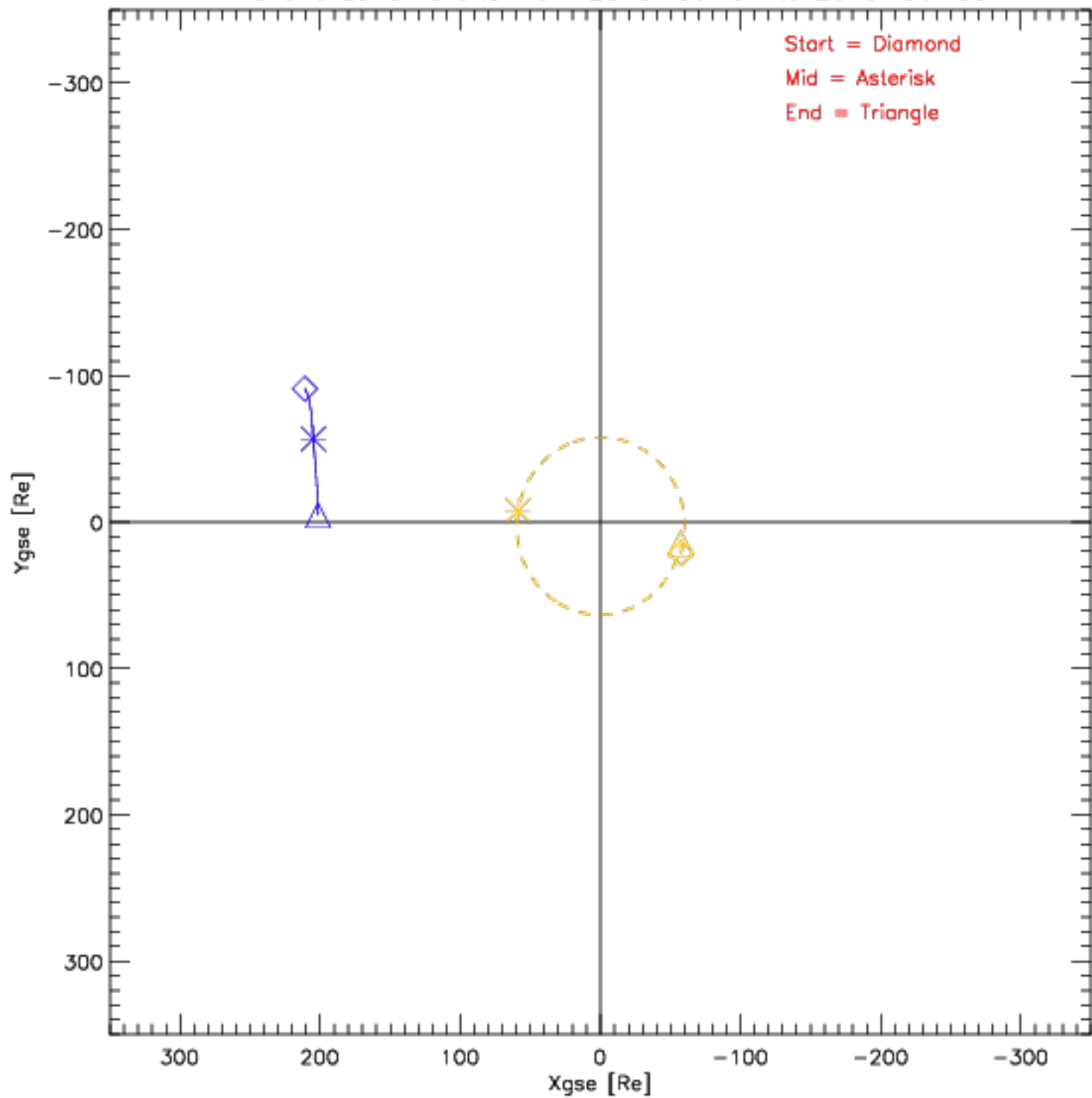
Wind and Lunar Orbits from 2015-06-01 to 2015-06-30
