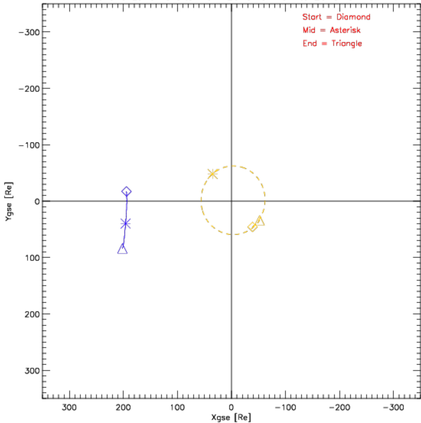
Wind and Lunar Orbits from 2015-01-01 to 2015-01-31
