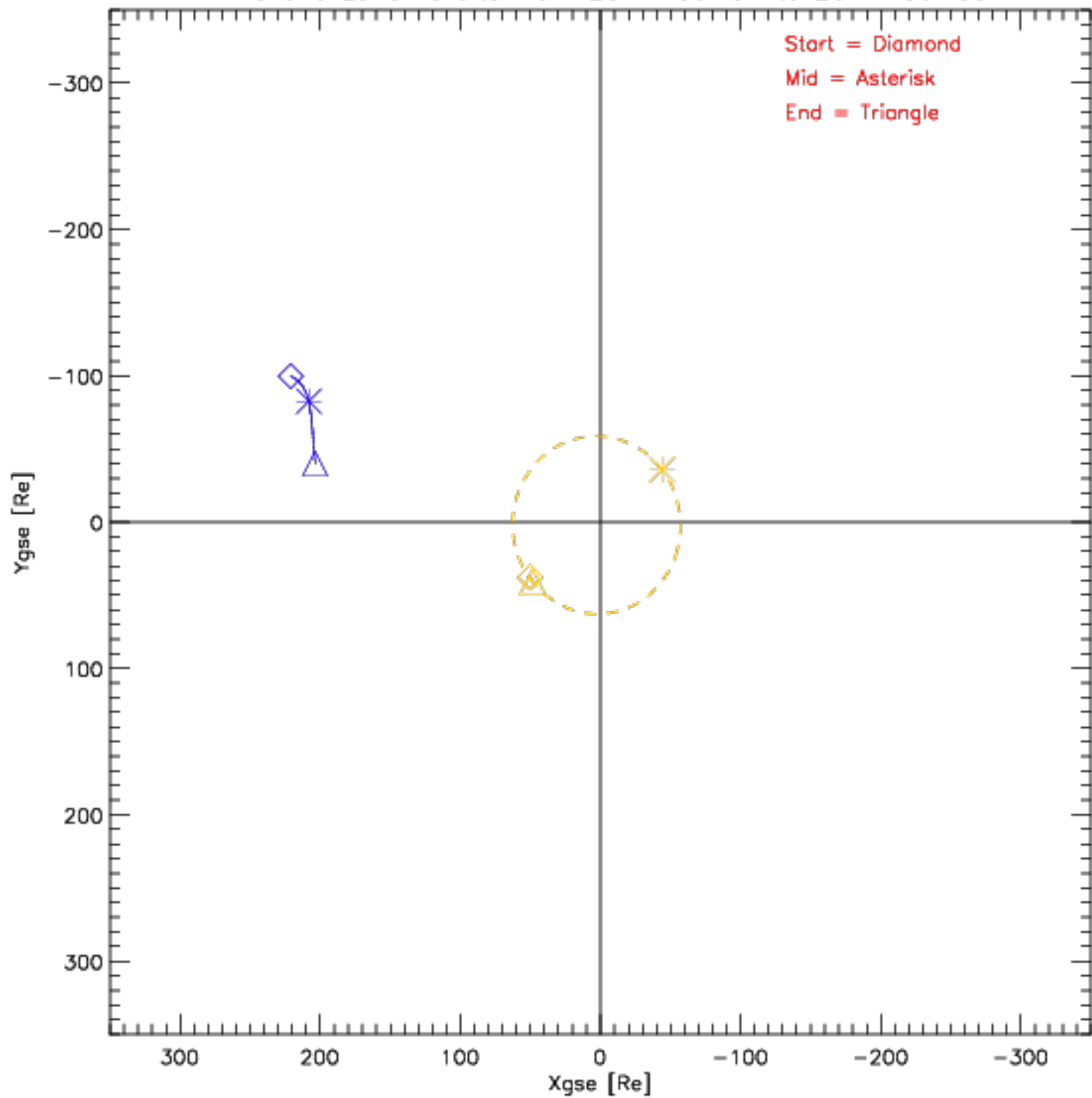
Wind and Lunar Orbits from 2014-06-01 to 2014-06-30
