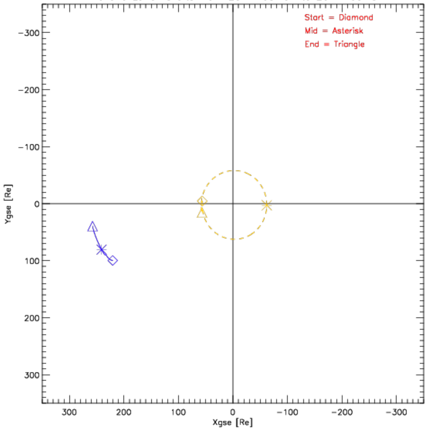
Wind and Lunar Orbits from 2014-03-01 to 2014-03-31
