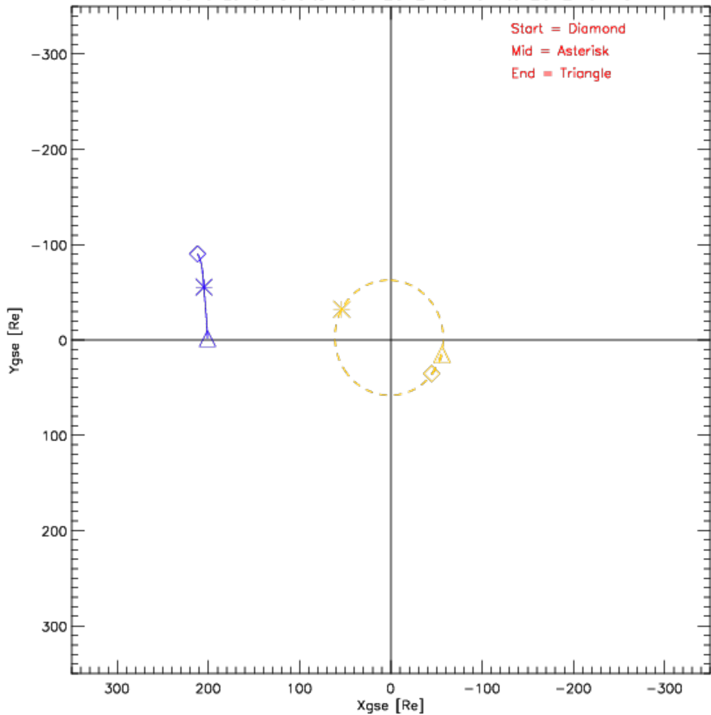
Wind and Lunar Orbits from 2012-07-01 to 2012-07-31
