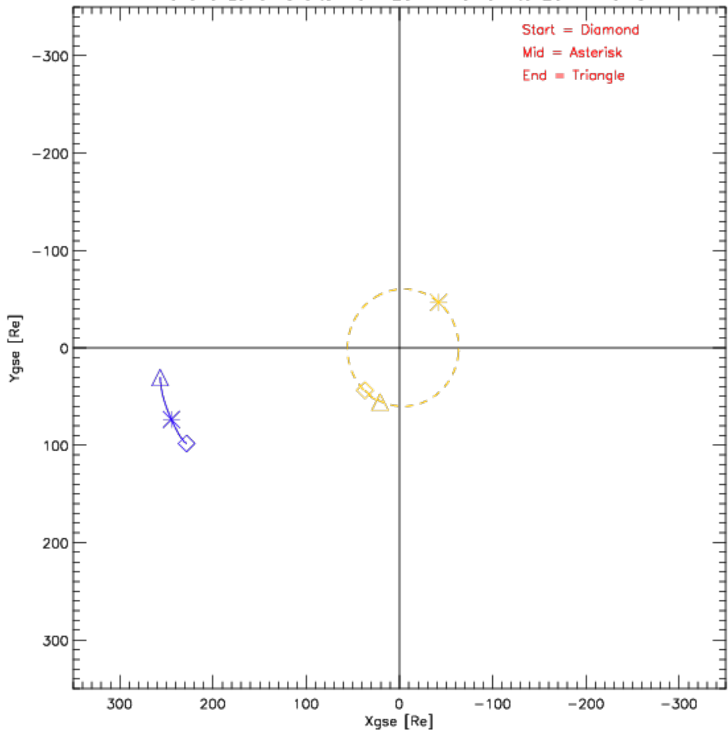
Wind and Lunar Orbits from 2011-10-01 to 2011-10-31
