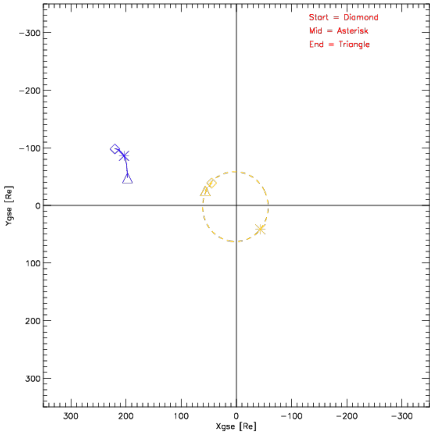
Wind and Lunar Orbits from 2011-01-01 to 2011-01-31
