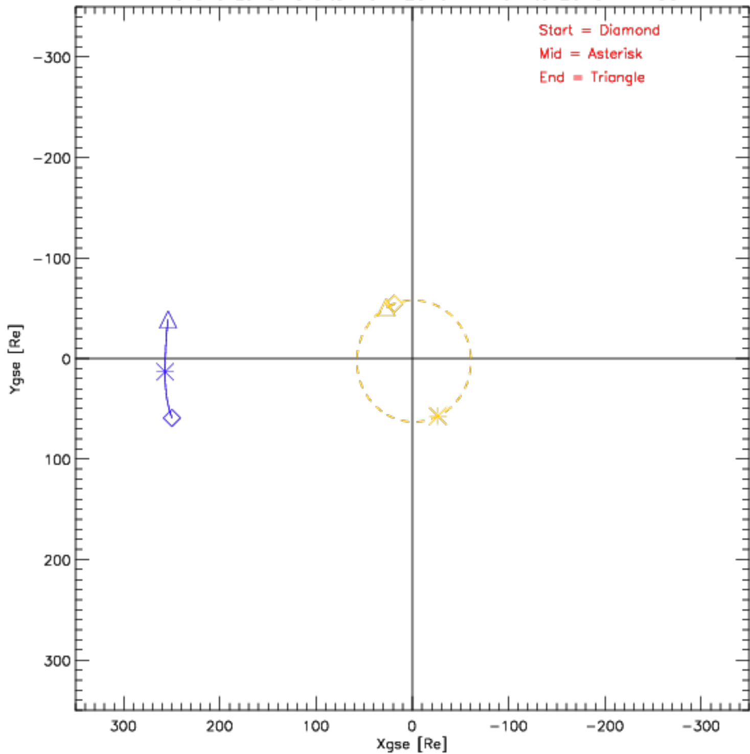
Wind and Lunar Orbits from 2010-11-01 to 2010-11-30
