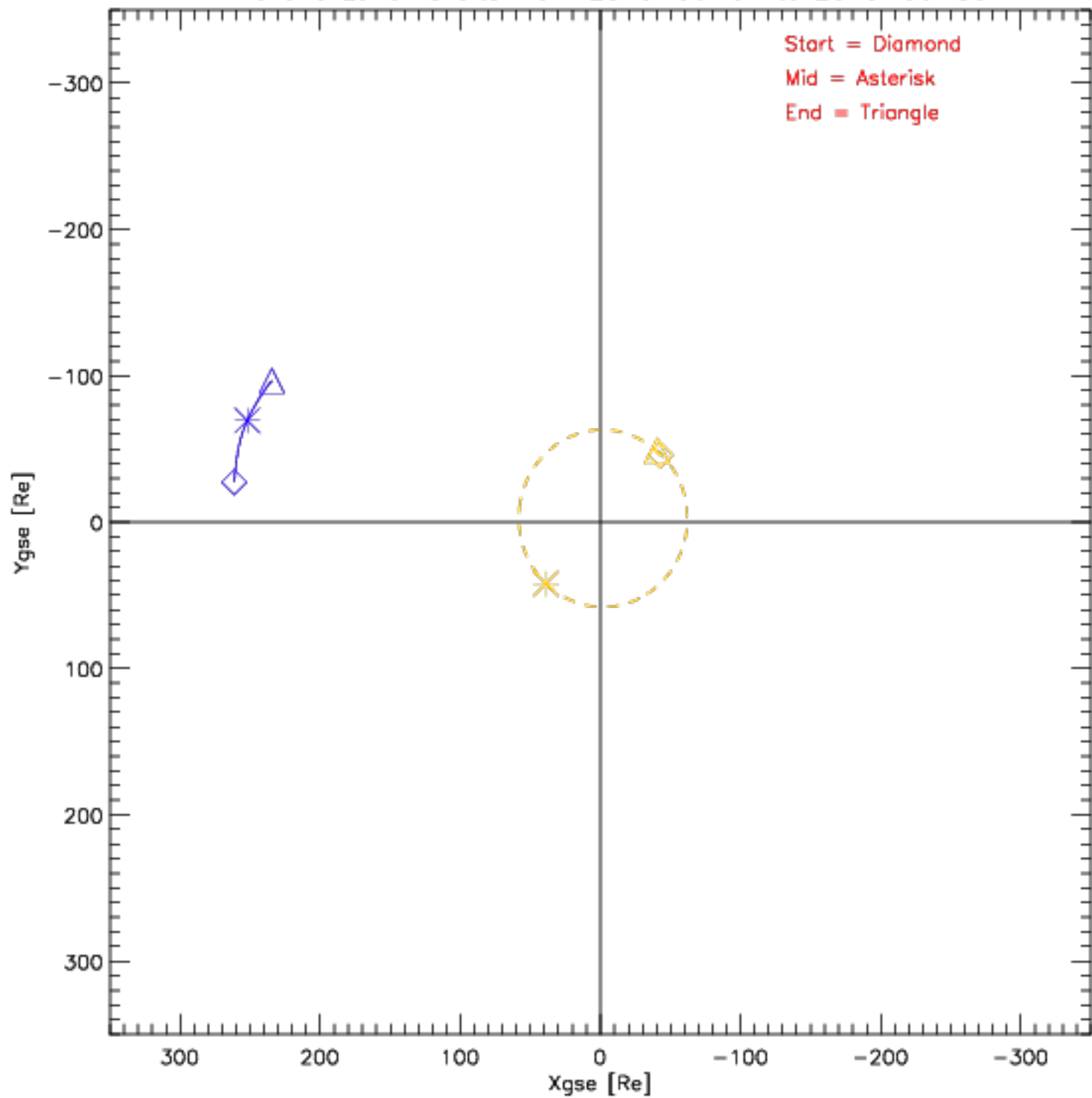
Wind and Lunar Orbits from 2010-06-01 to 2010-06-30
