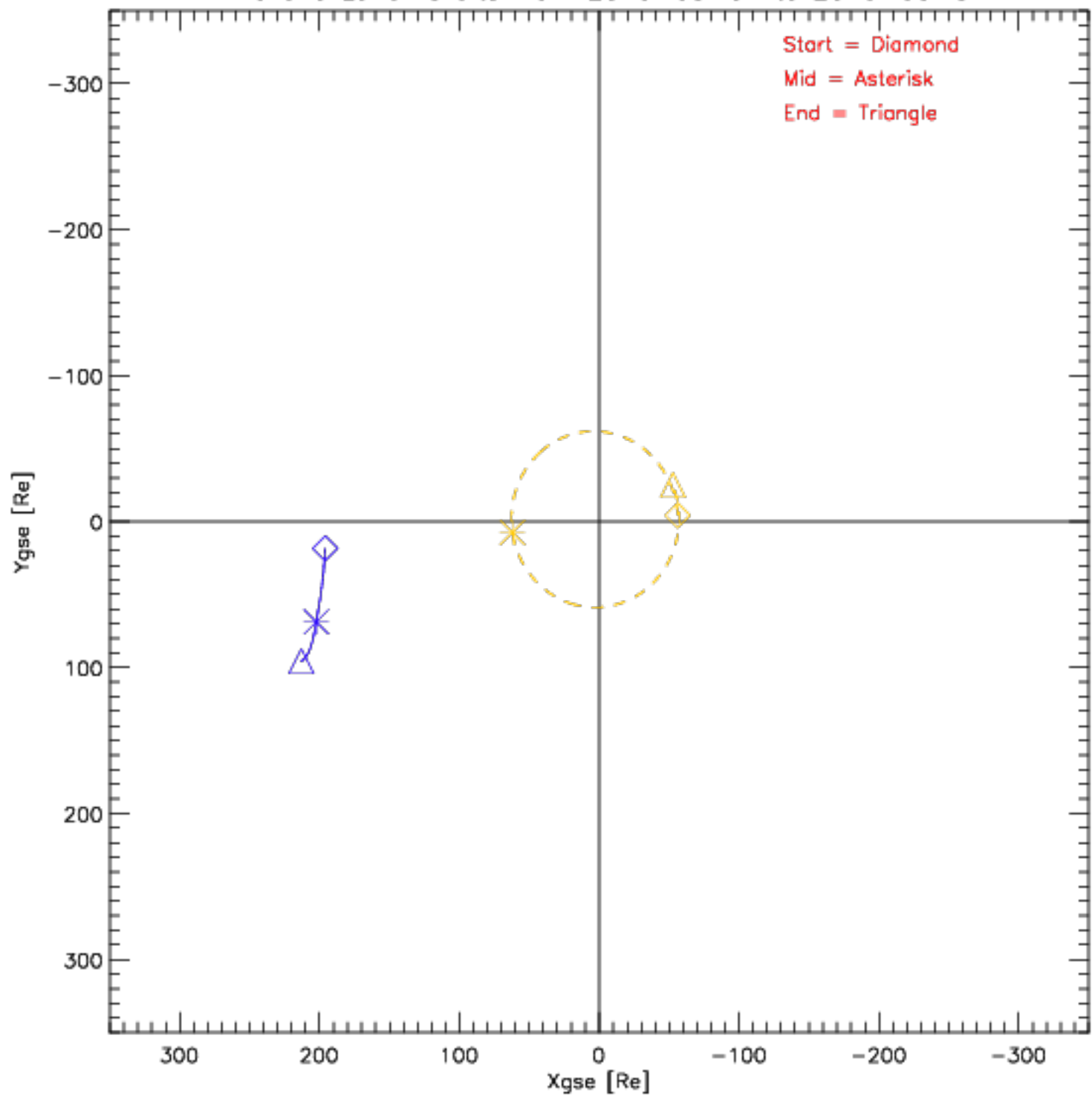
Wind and Lunar Orbits from 2010-03-01 to 2010-03-31
