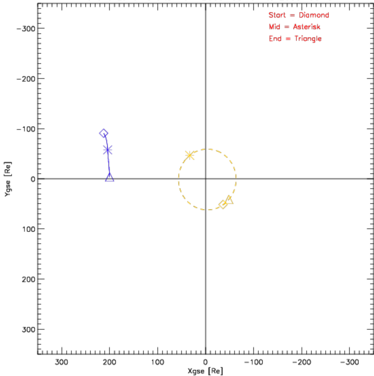
Wind and Lunar Orbits from 2009-08-01 to 2009-08-31
