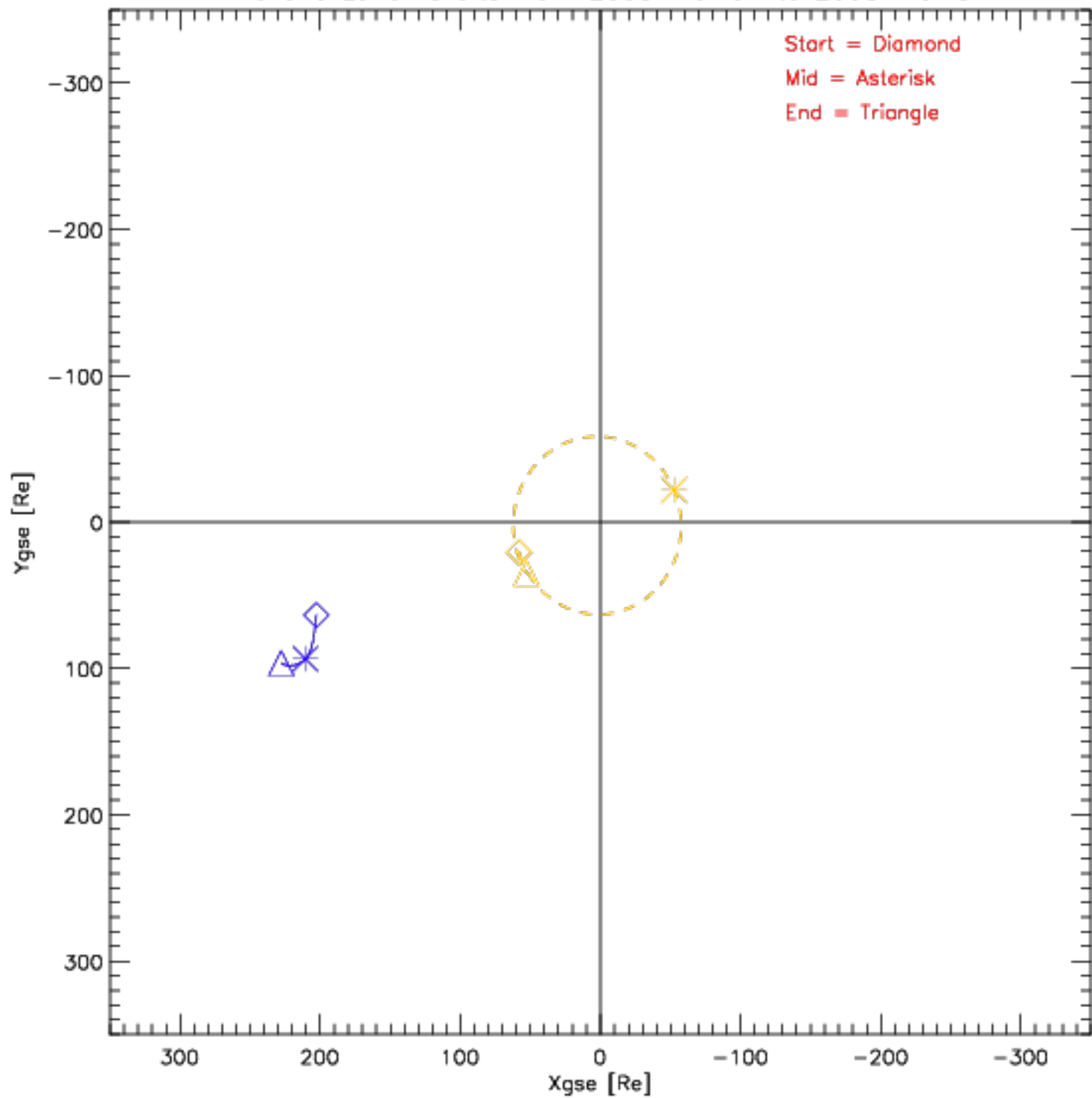
Wind and Lunar Orbits from 2008-10-01 to 2008-10-31
