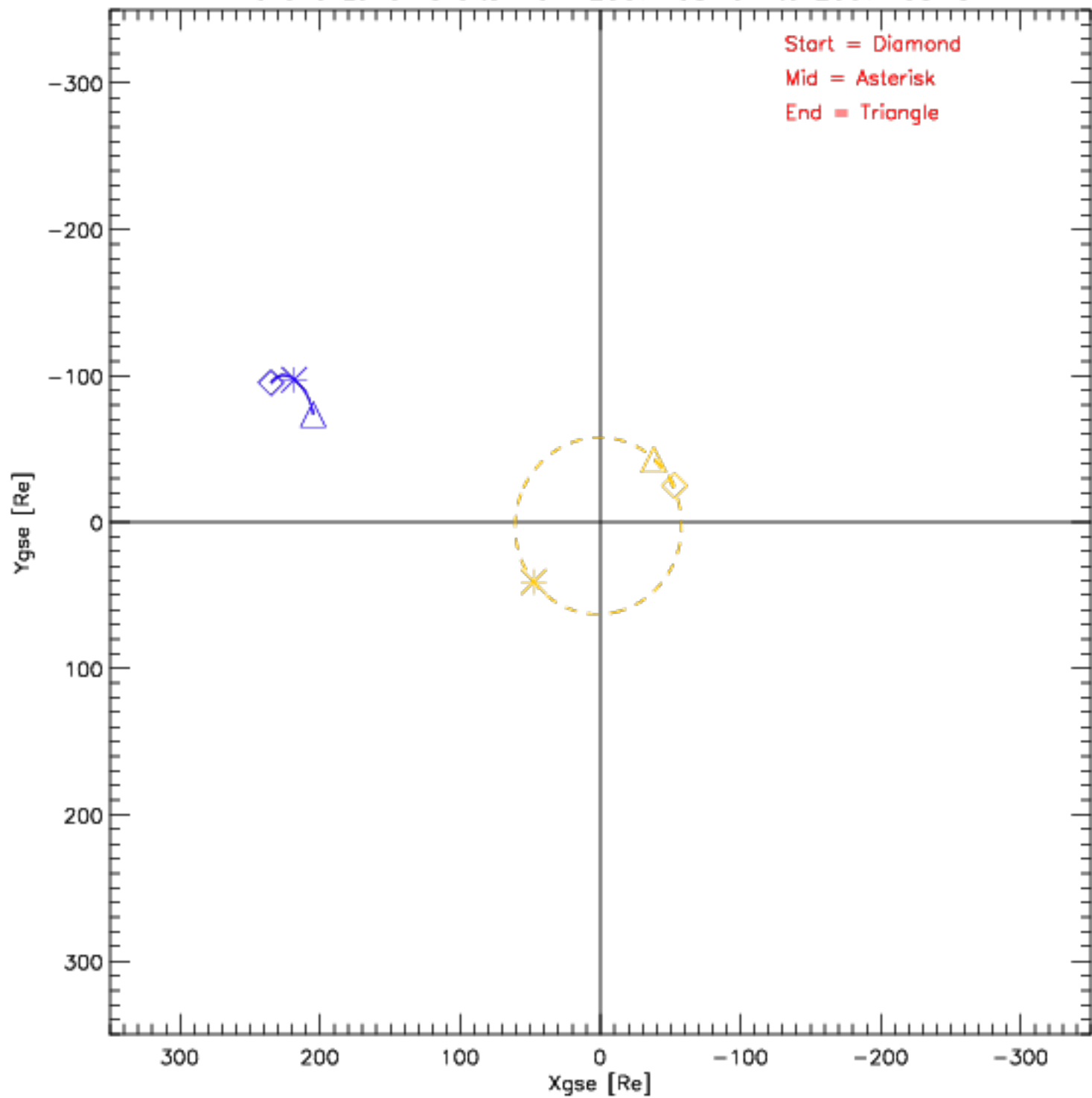
Wind and Lunar Orbits from 2007-08-01 to 2007-08-31
