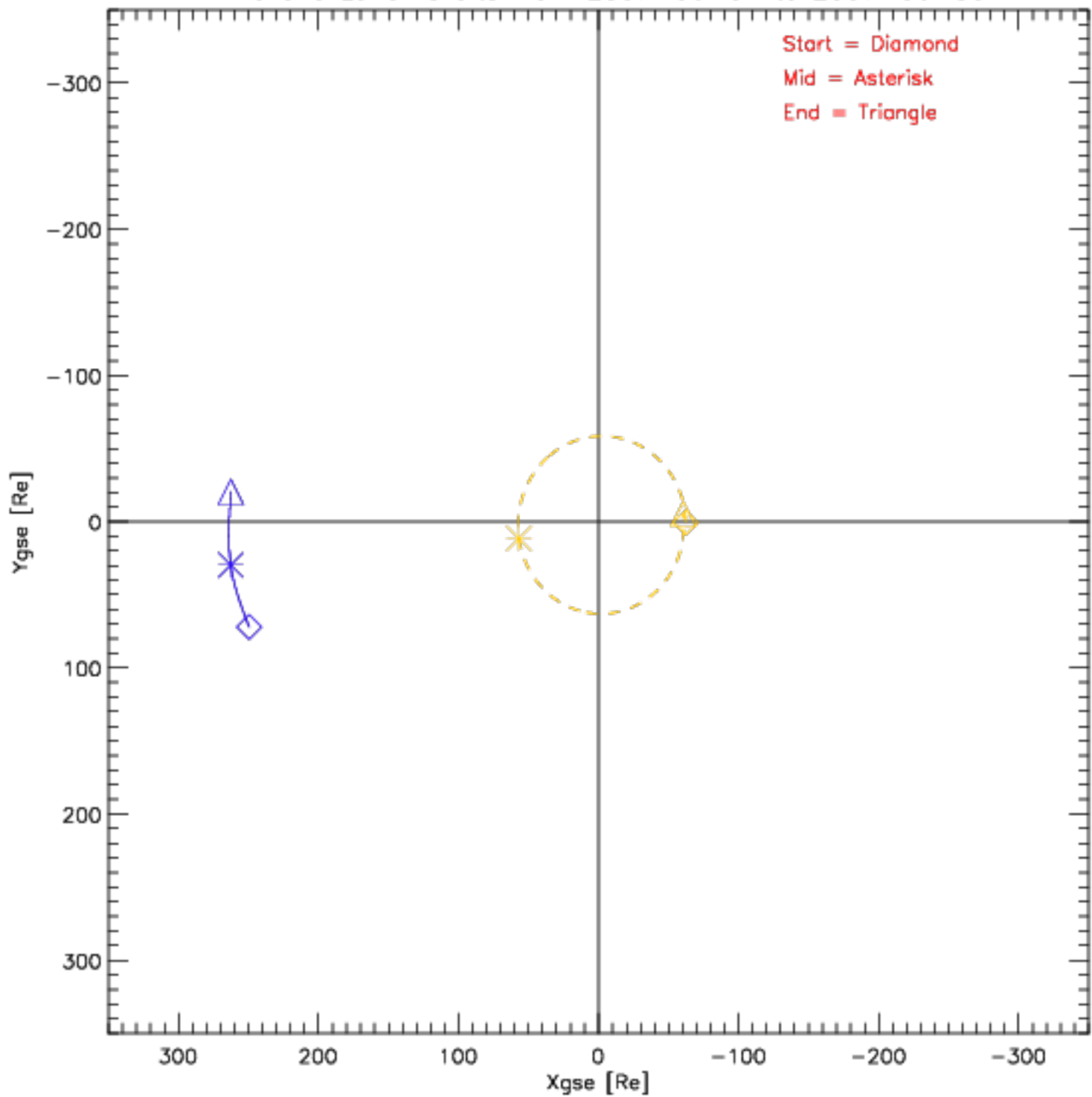
Wind and Lunar Orbits from 2007-06-01 to 2007-06-30
