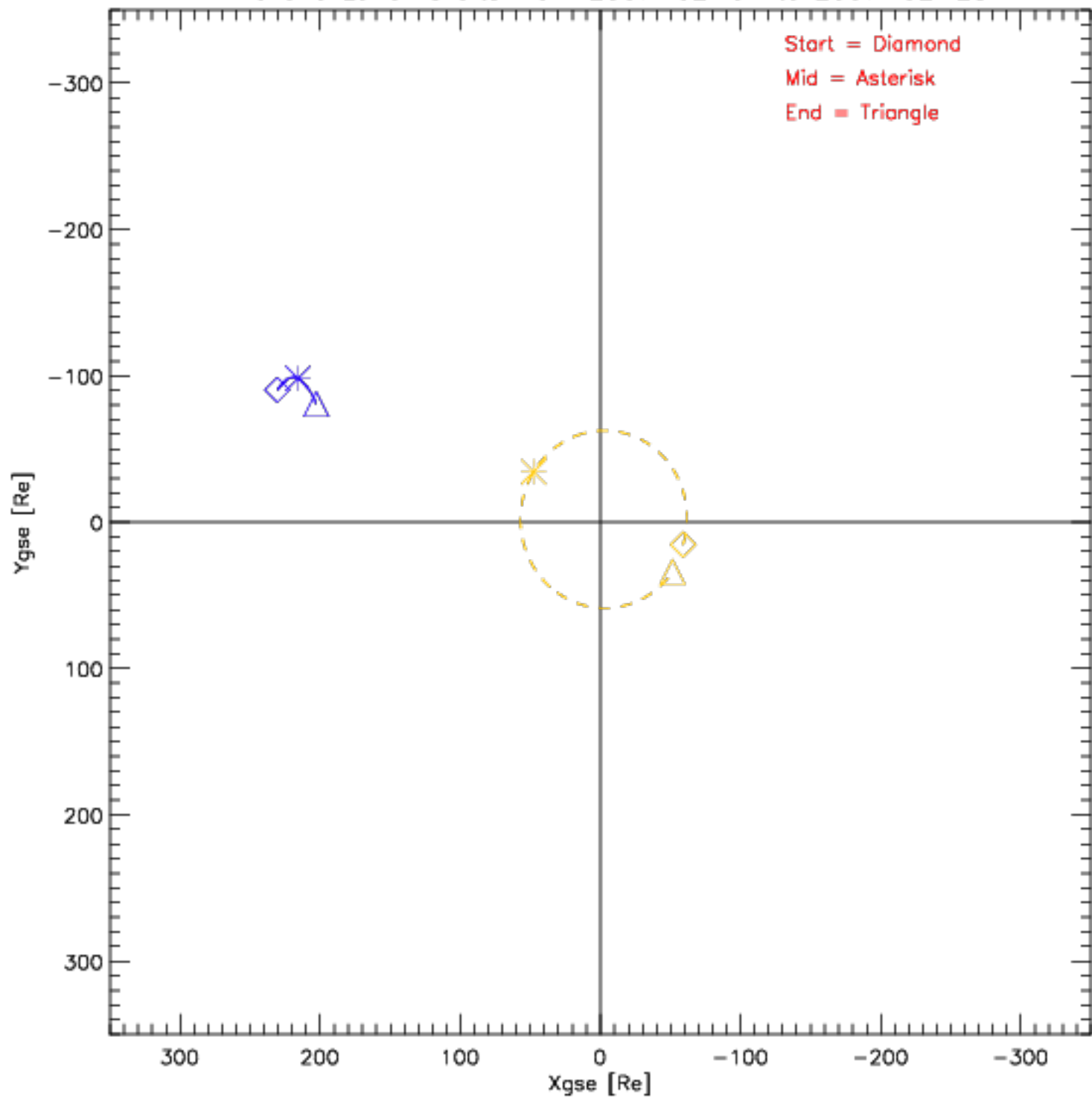
Wind and Lunar Orbits from 2007-02-01 to 2007-02-28
